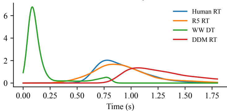
Older density
