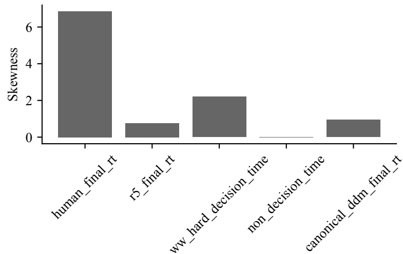
Older skewness
