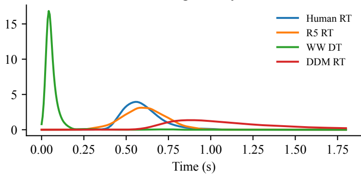
Young density
