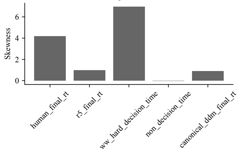
Young skewness
