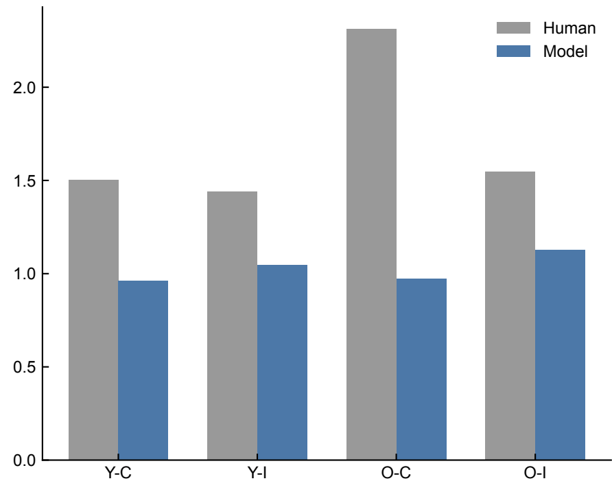
Skew-like index
