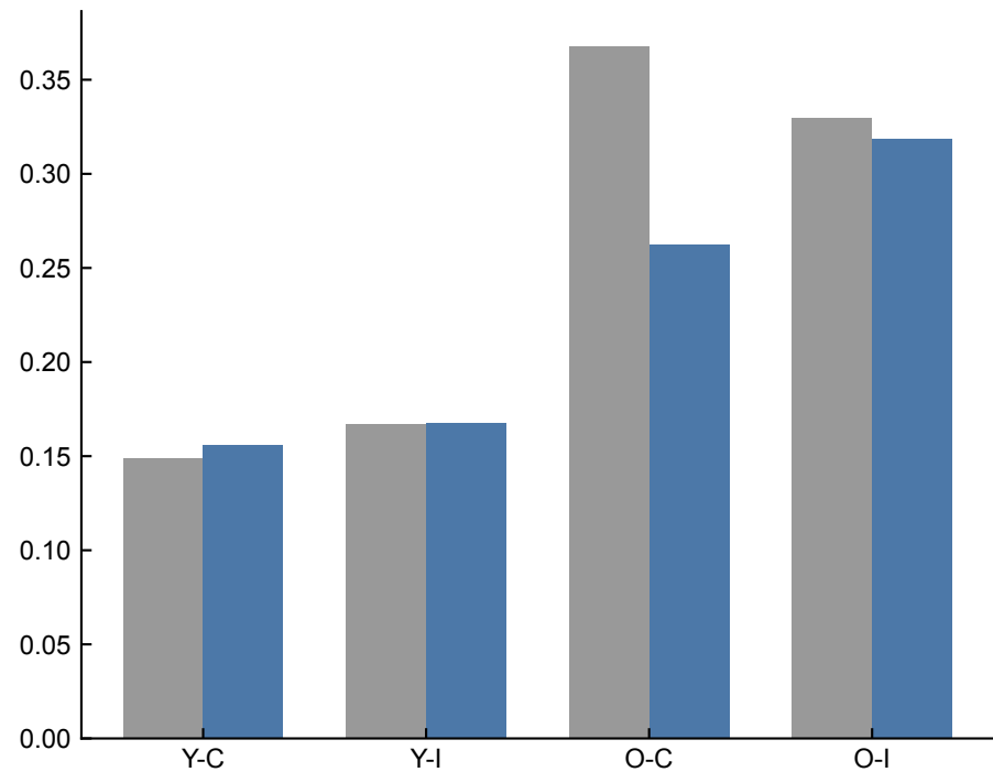
Tail index
