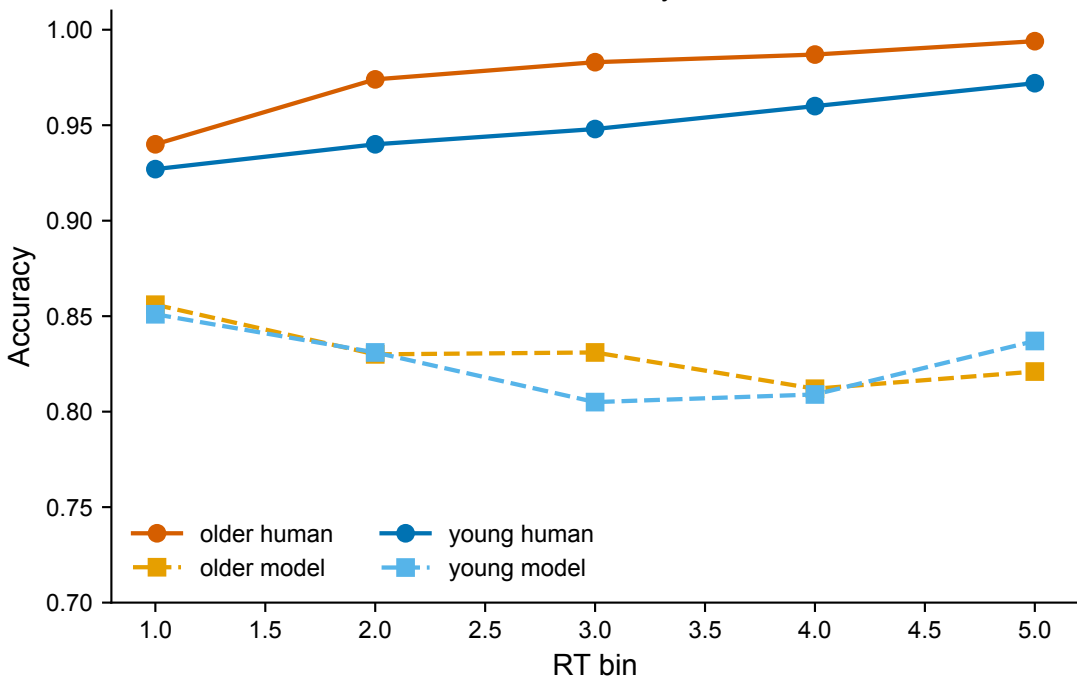
Conditional accuracy function
