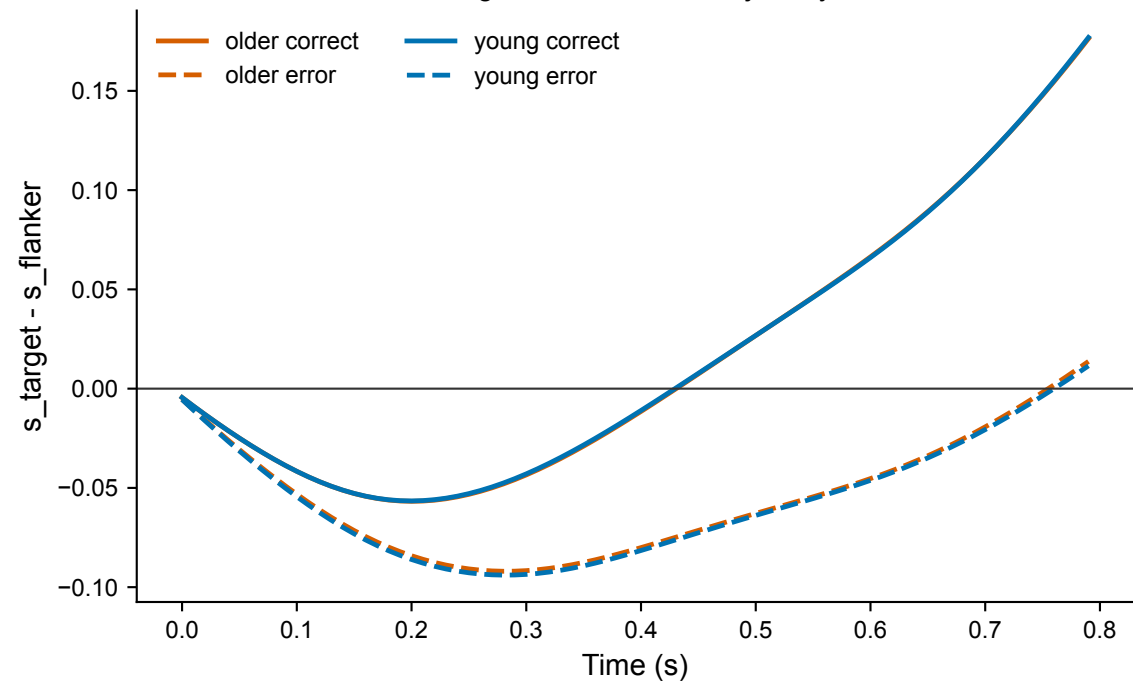
Target-minus-flanker trajectory
