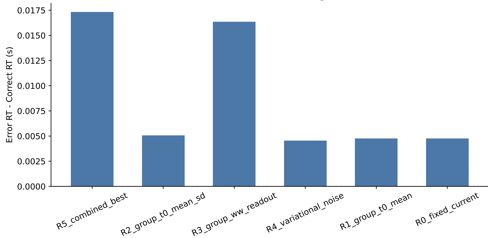
Error-minus-correct RT across existing model families
