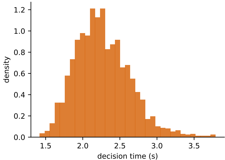
rtify_4choice_calibrated_noise_dt10, gap=0.1
