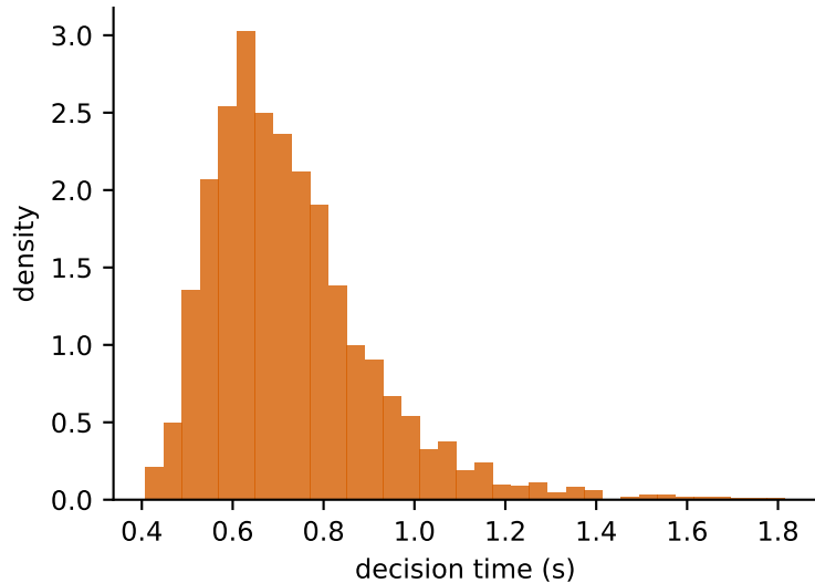
ww_2choice_dt1, gap=0.0
