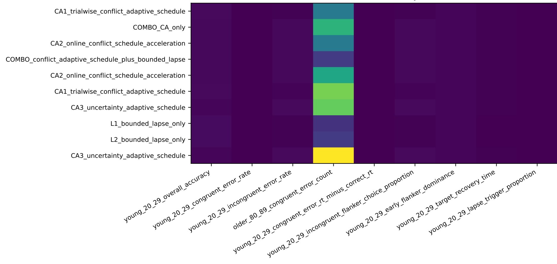
Mechanism tradeoff summary dashboard
