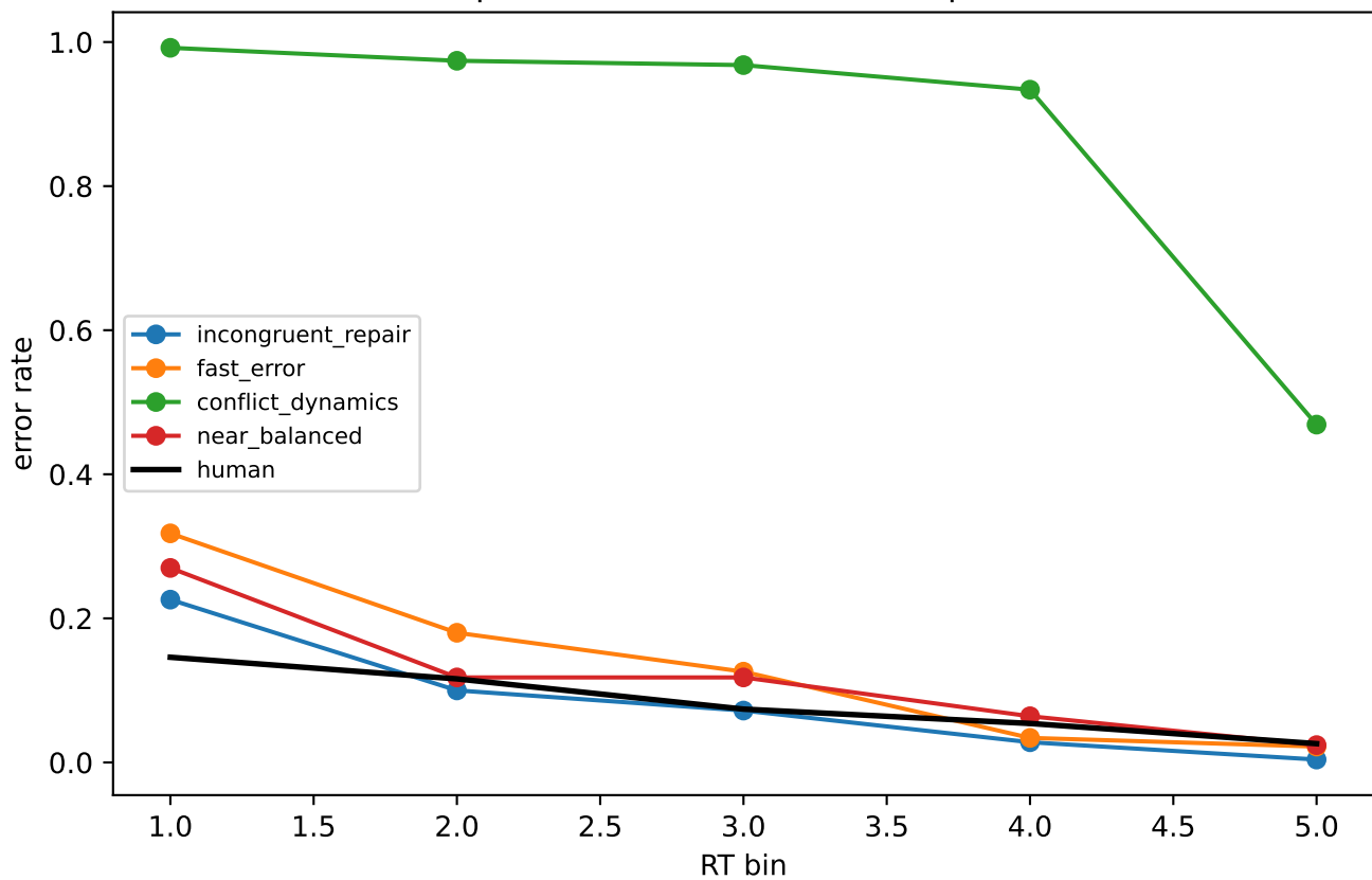
Representative models RT-bin profile
