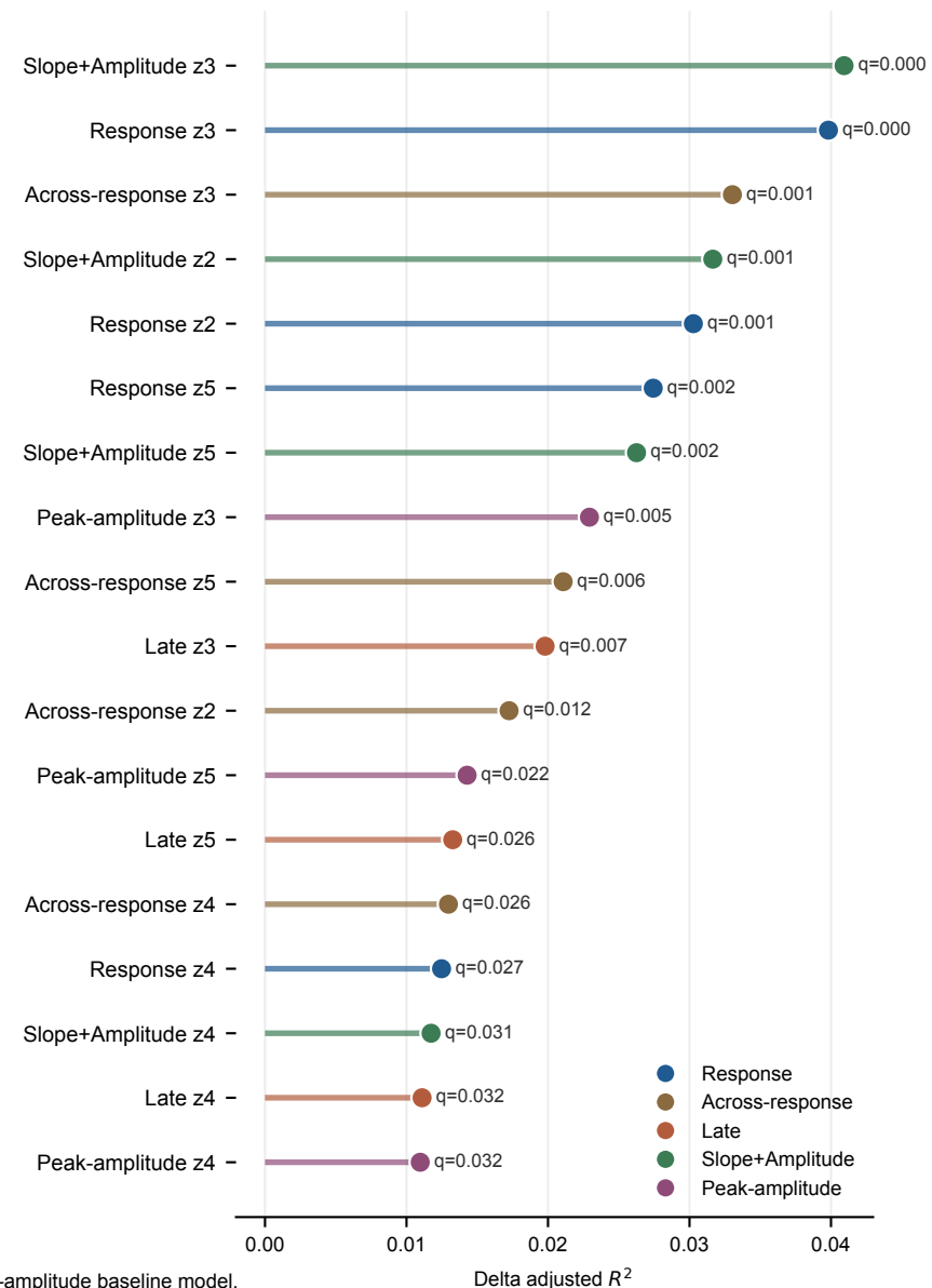
b FDR-significant latent additions
