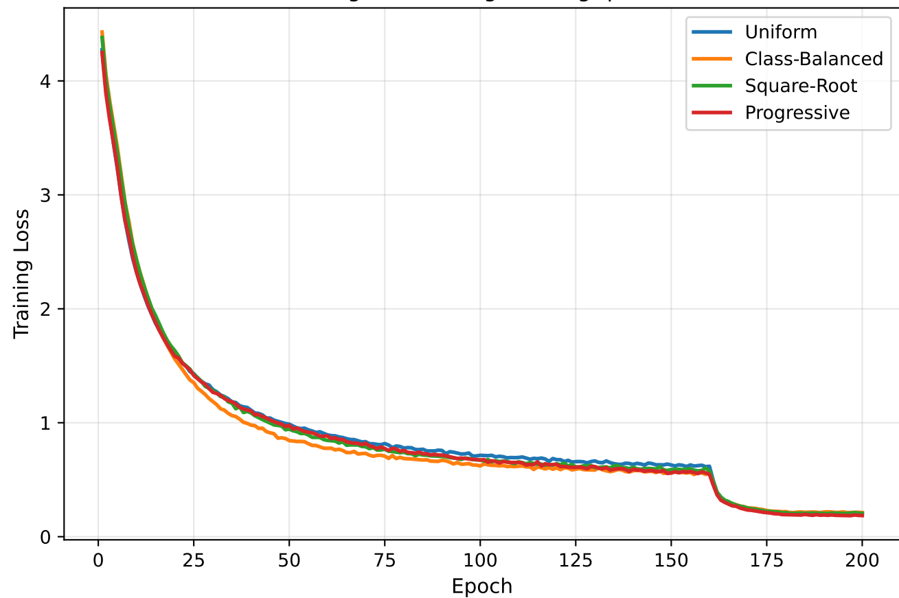
Training Loss During Training ( \rho = 10 )
