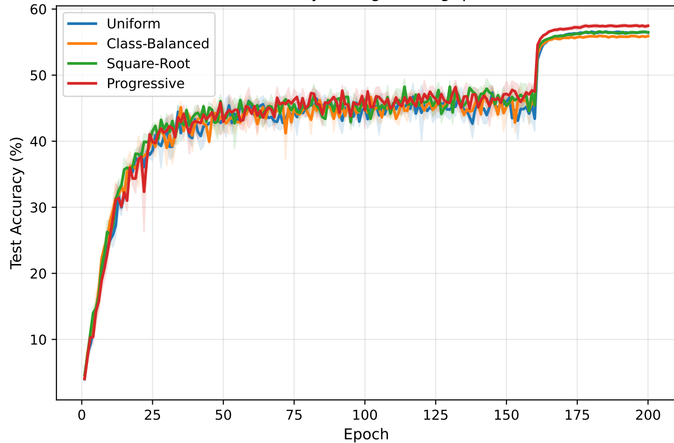
Test Accuracy During Training ( \rho = 10 )
