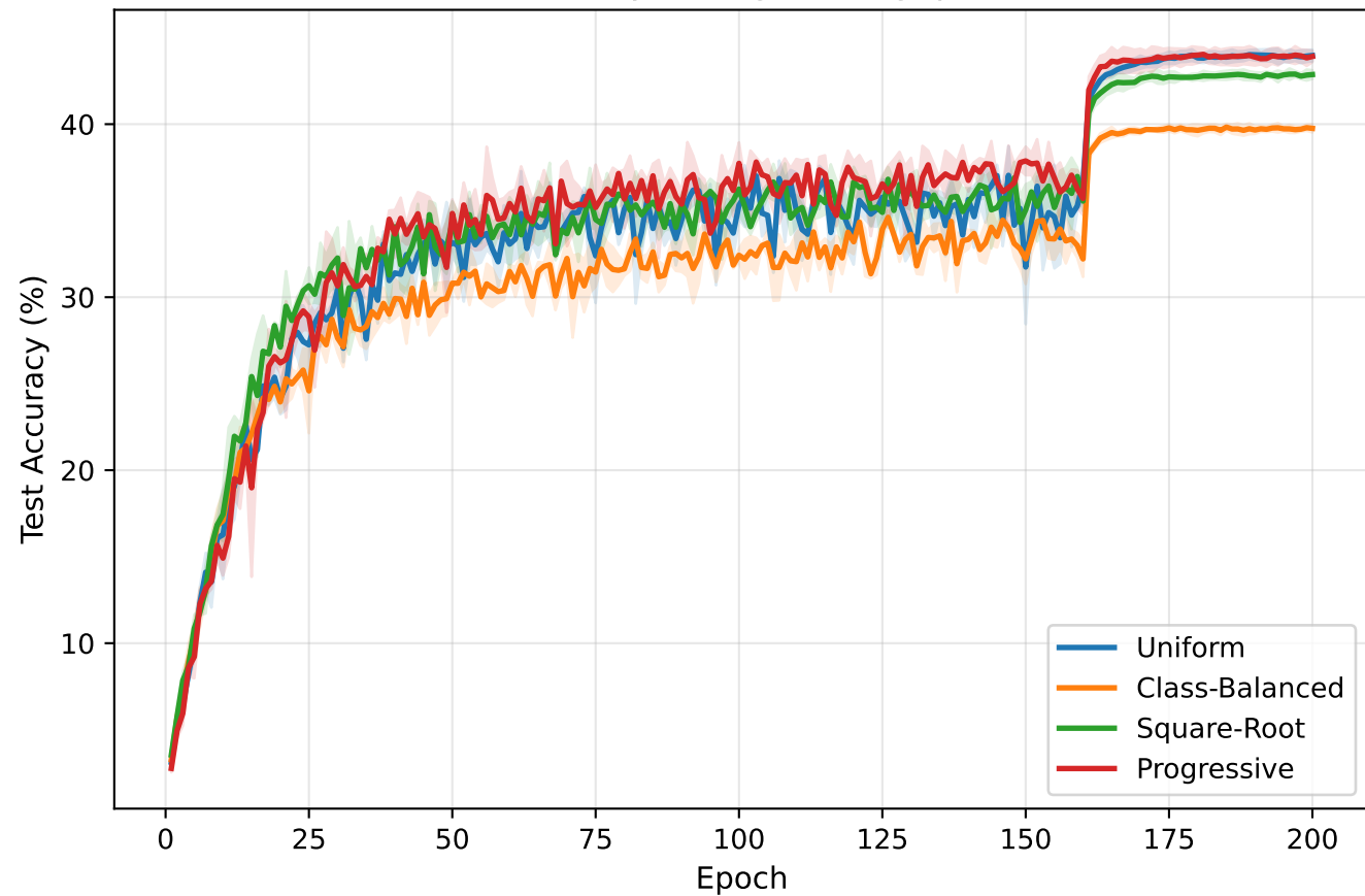
Test Accuracy During Training ( \rho = 50 )
