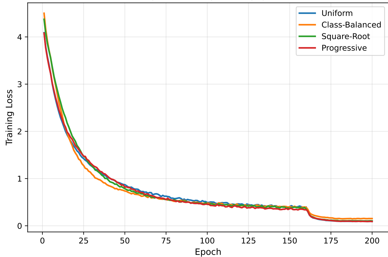
Training Loss During Training ( \rho = 50 )
