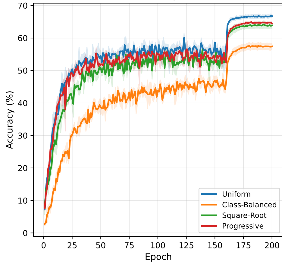
Head Classes ( \rho = 100 )
