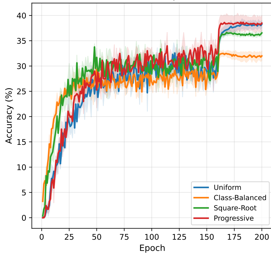
Medium Classes ( \rho = 100 )
