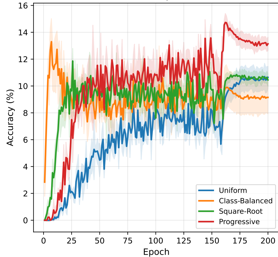
Tail Classes ( \rho = 100 )
