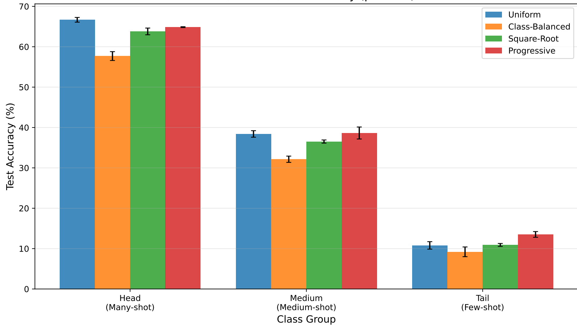
Head/Medium/Tail Accuracy ( \rho = 100 )
