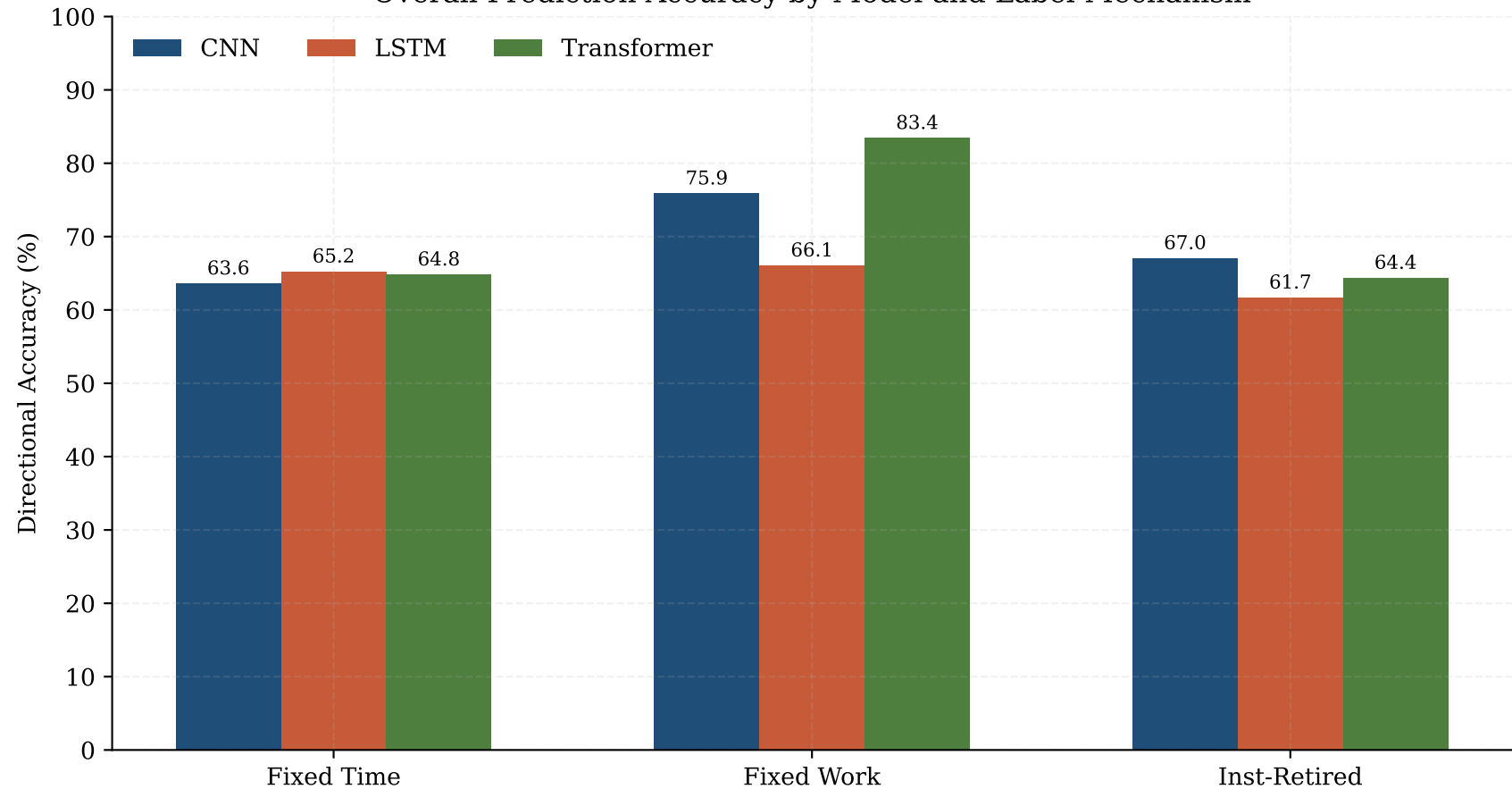
Overall Prediction Accuracy by Model and Label Mechanism
