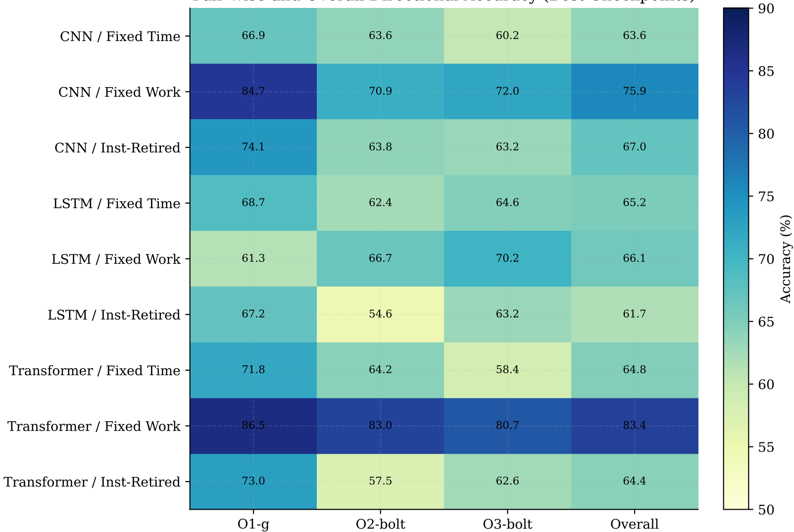
Pair-wise and Overall Directional Accuracy (Best Checkpoints)
