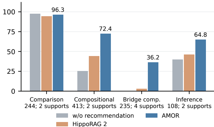
(a) Evidence dependencies matter All 1,000 2Wiki questions
