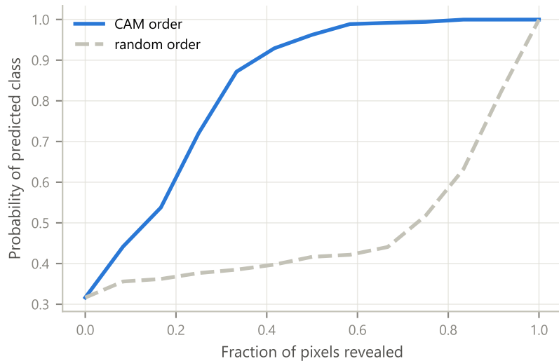
(b) Insertion — AUC 0.841 vs 0.482 passes (higher is better)
