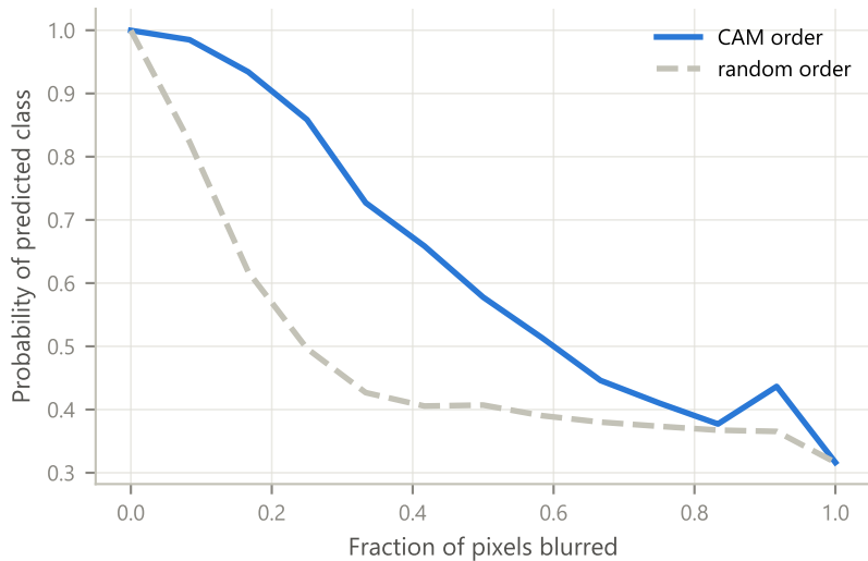
(a) Deletion — AUC 0.632 vs 0.476 FAILS (lower is better)
