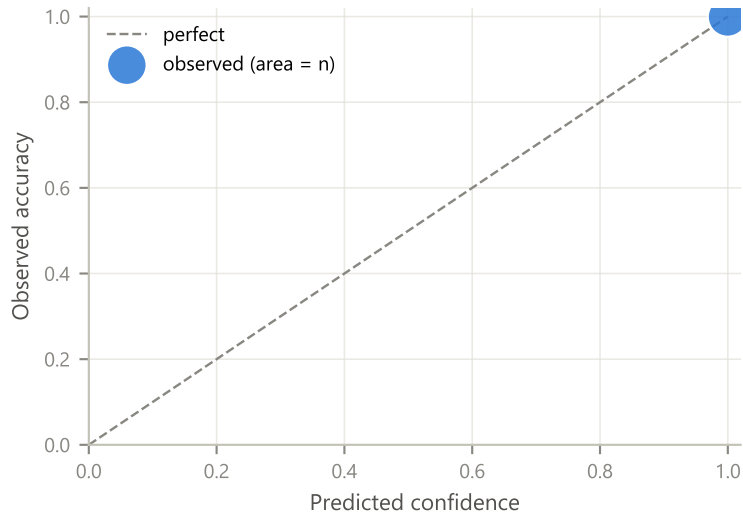
(b) Temperature-scaled ( T = 0.426 ) ECE = 0.0011
