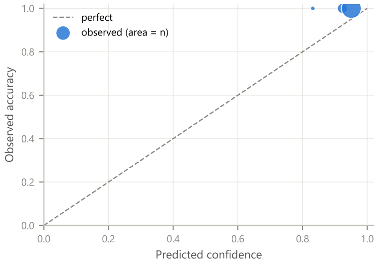
(a) Uncalibrated ECE = 0.0503
