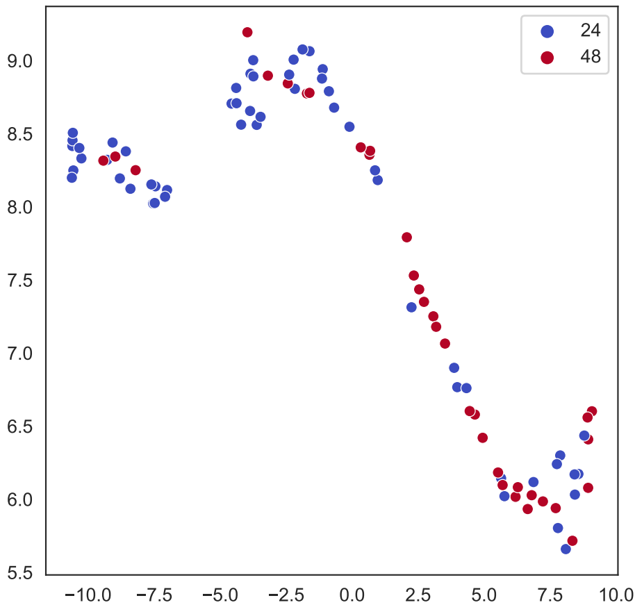
UMAP 10 neighbors
