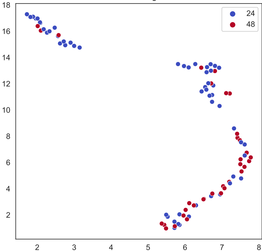
UMAP 15 neighbors
