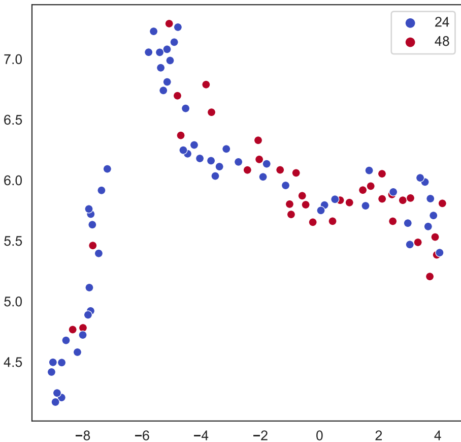
UMAP 20 neighbors
