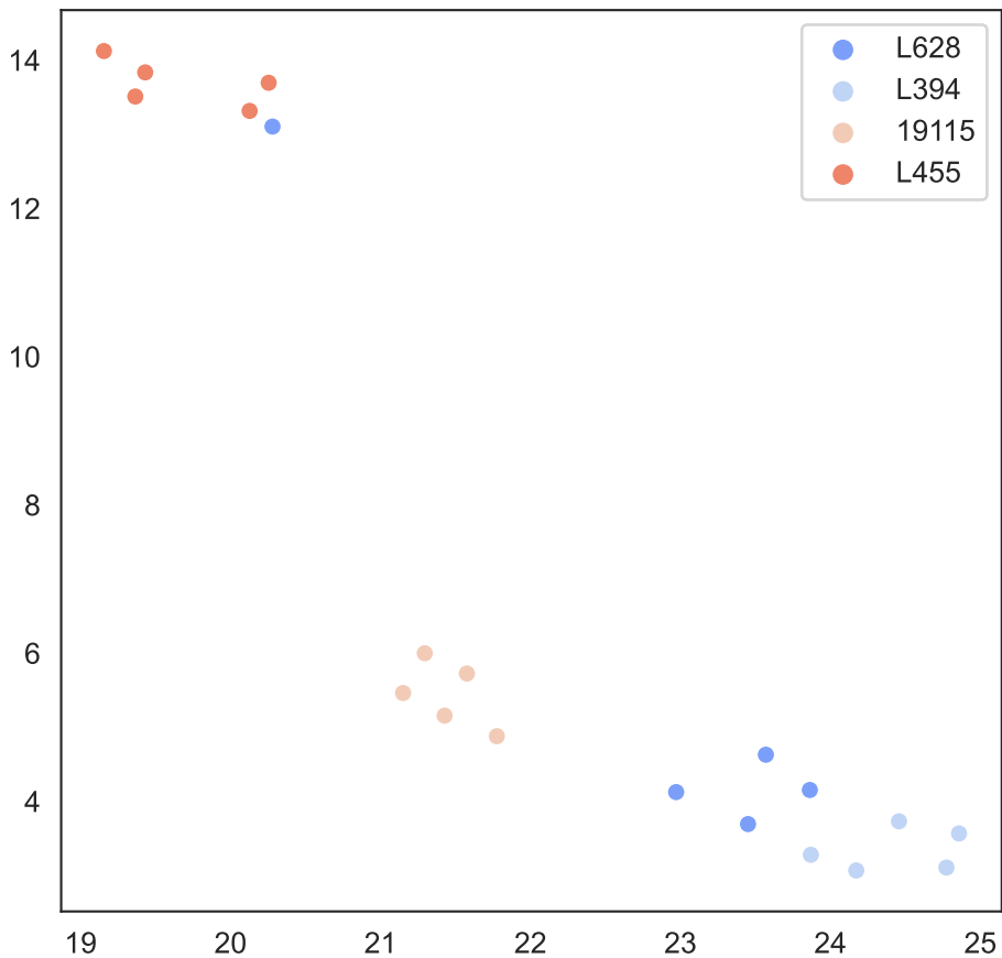
UMAP 5 neighbors
