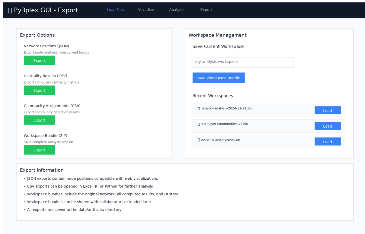
Figure 4: Export page for saving analysis results and workspace bundles
