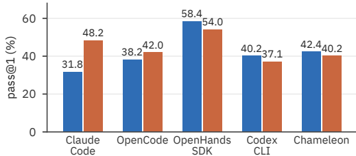
SWE-bench Verified
