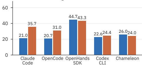
SWE-bench Multilingual
