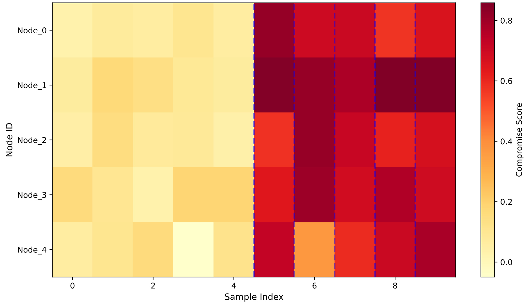
Attribution Heatmap: Compromise Probability per Node
