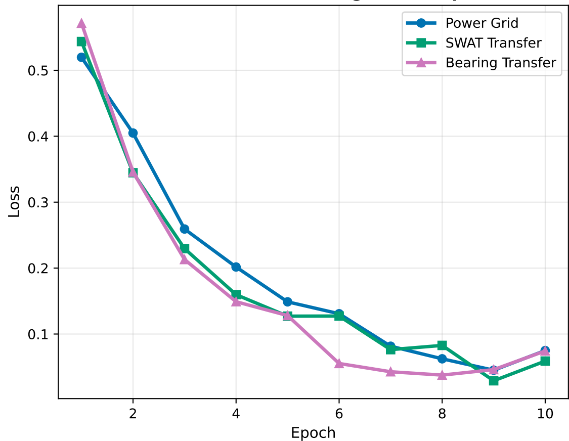
Multi-Domain: Loss Convergence Comparison
