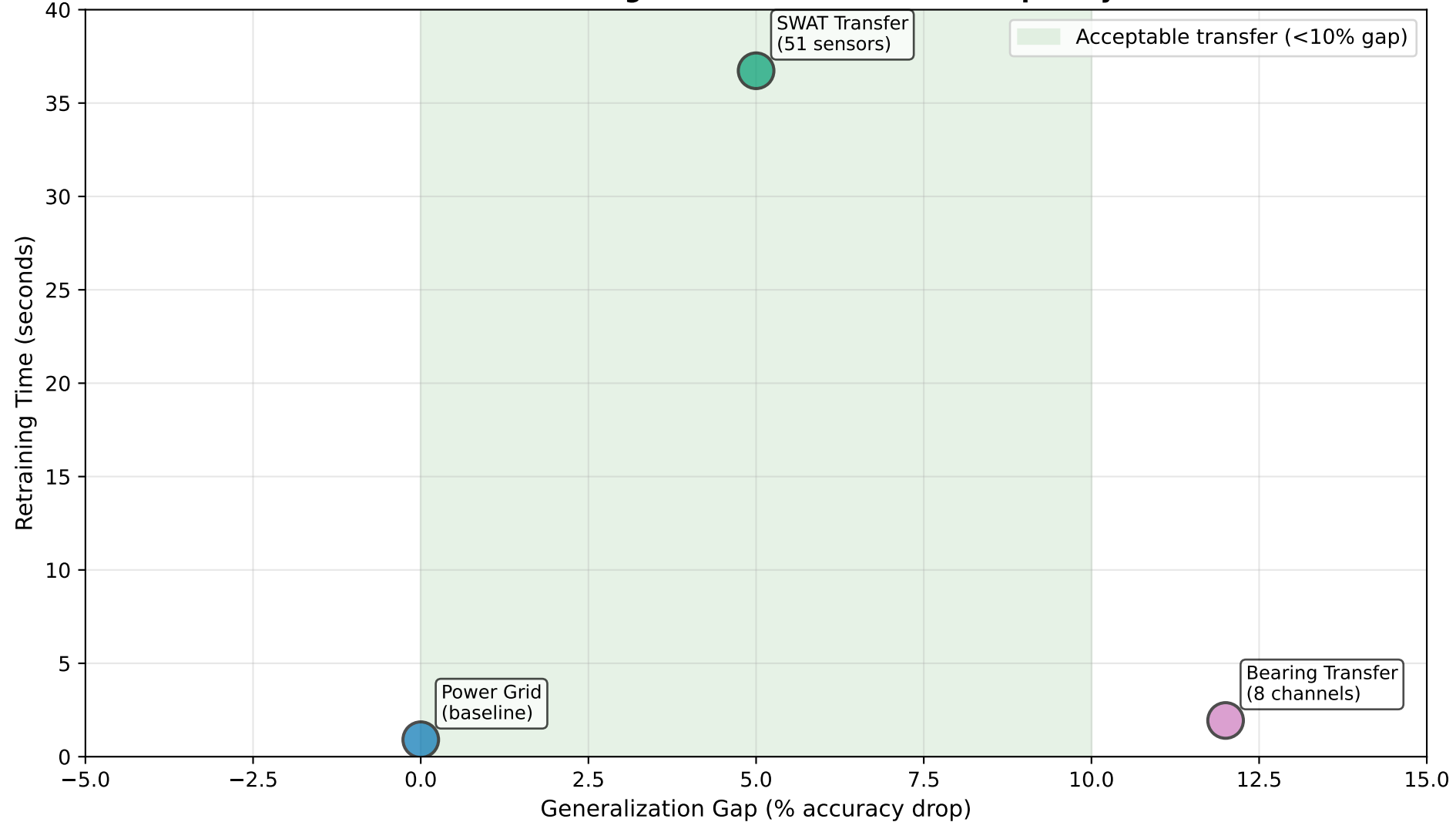
Transfer Learning Cost: Time vs Domain Complexity
