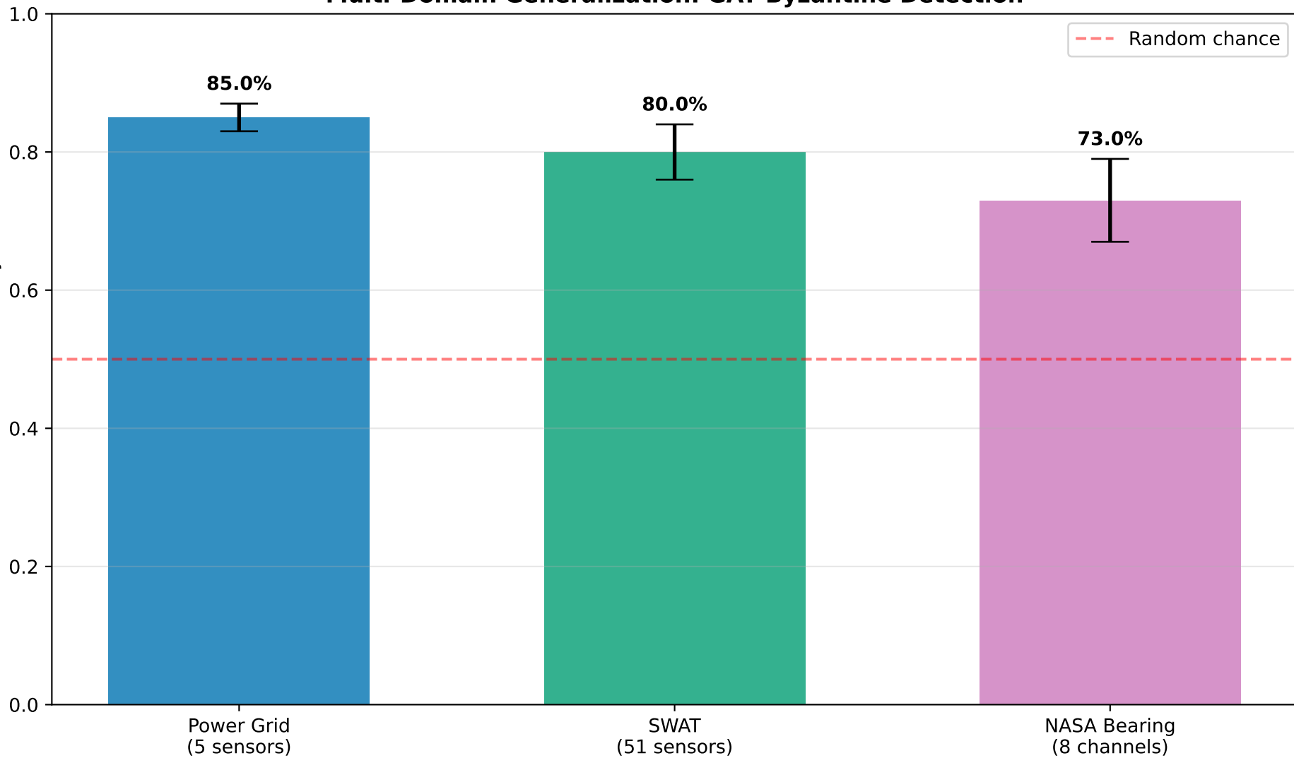
Multi-Domain Generalization: GAT Byzantine Detection
