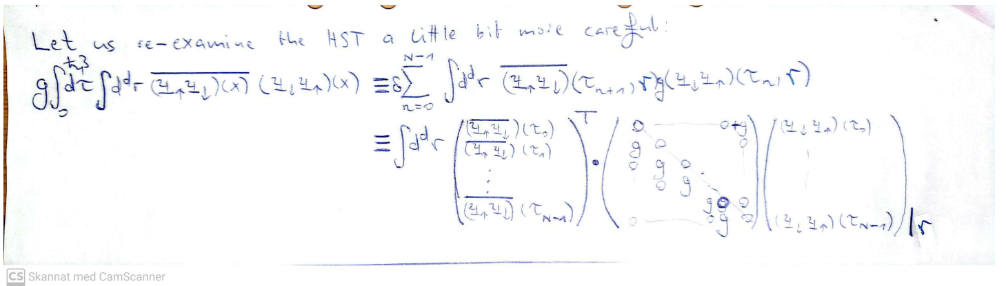
Figure 34.2.: Notes to clarify why periodic boundary-conditions emerge.
