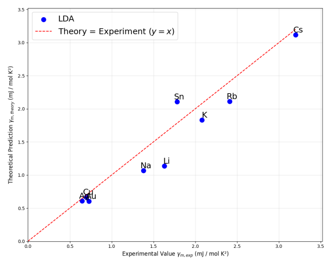
Figure 23.2.: Specific heat of various materials contrasting LDA and Experimental Results. Produced with quantum espresso v7.2 and norm conserving pseudopotentials from sssp.
