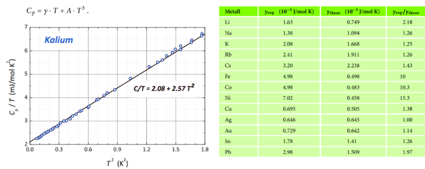
Figure 23.1.: Specific heat of various materials at low temperatures, taken from [19].
