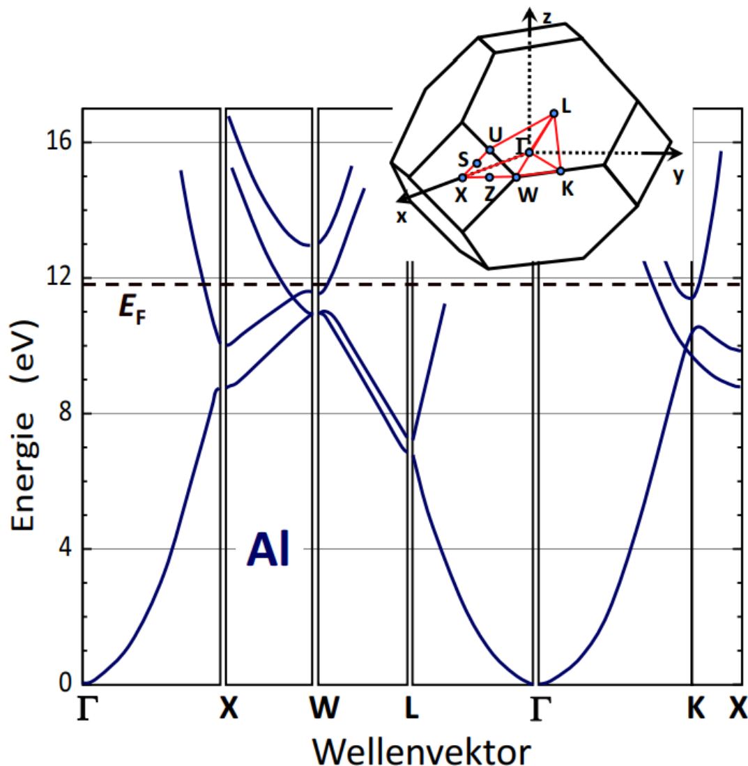
Figure 22.1.: The Band-Structure of Aluminium along the high-symmetry \mathbf{k} -points. Taken from [19].
