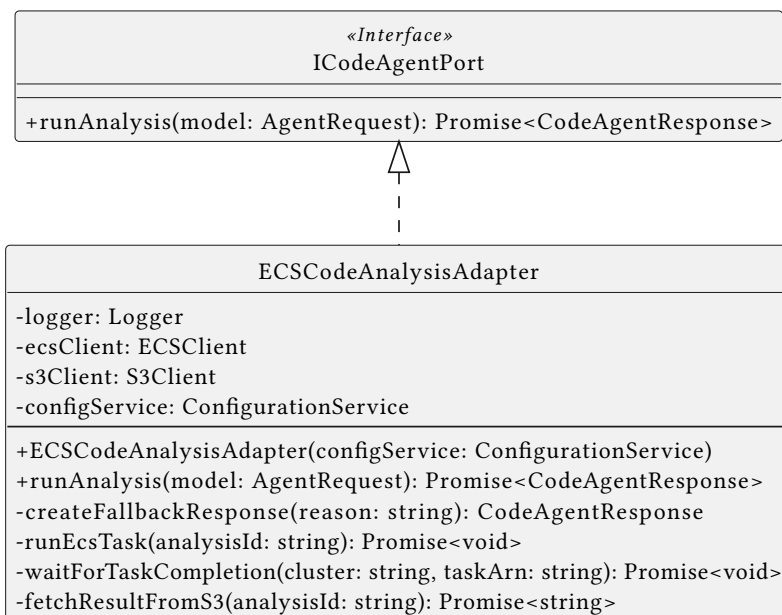
Figure 163: Class Diagram — ECSCodeAnalysisAdapter
