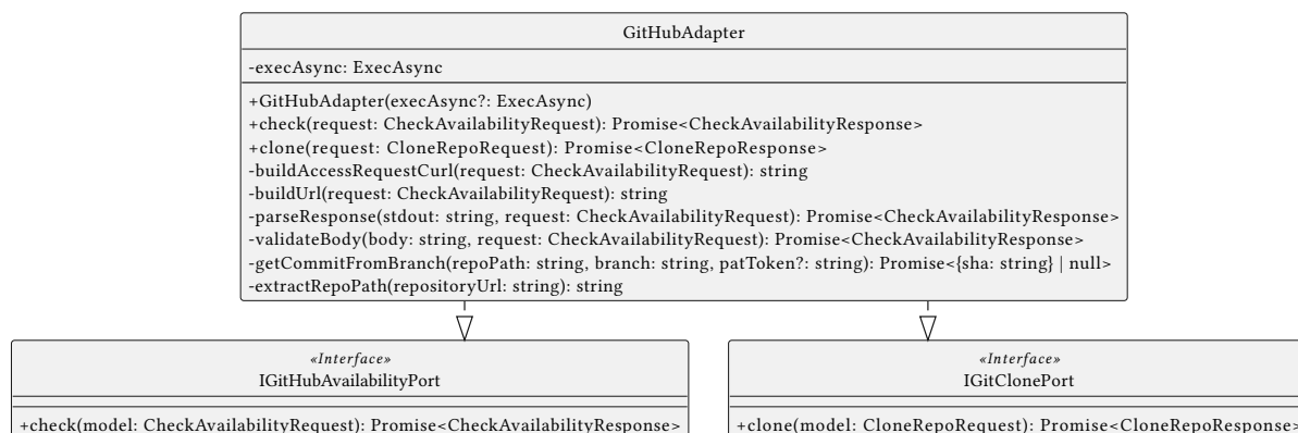
Figure 157: Class Diagram — GitHubAdapter
