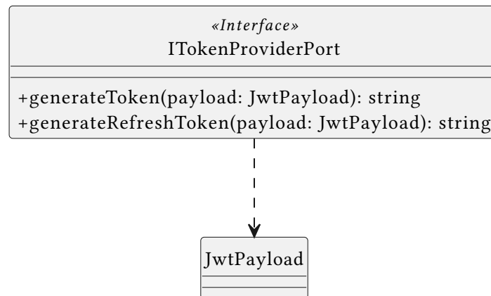
Figure 215: Class Diagram — ITokenProviderPort
