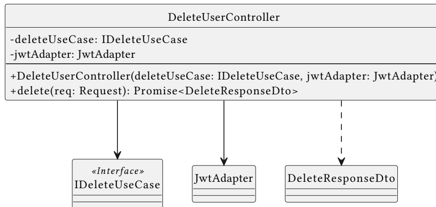
Figure 234: Class Diagram – DeleteUserController
