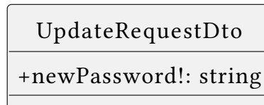
Figure 242: Class Diagram — UpdateRequestDto
