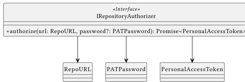
Figure 85: Class Diagram – IRepositoryAuthorizer
