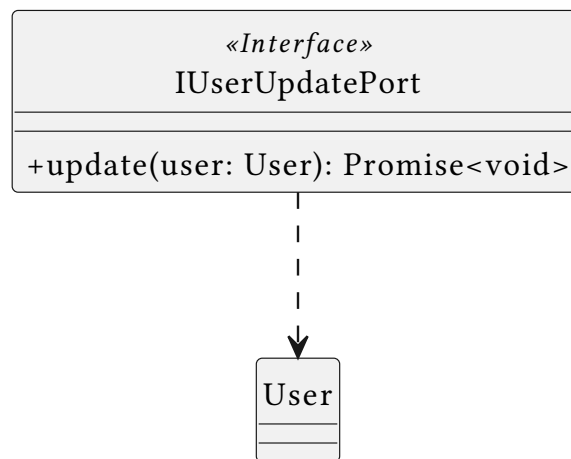
Figure 219: Class Diagram — IUserUpdatePort
