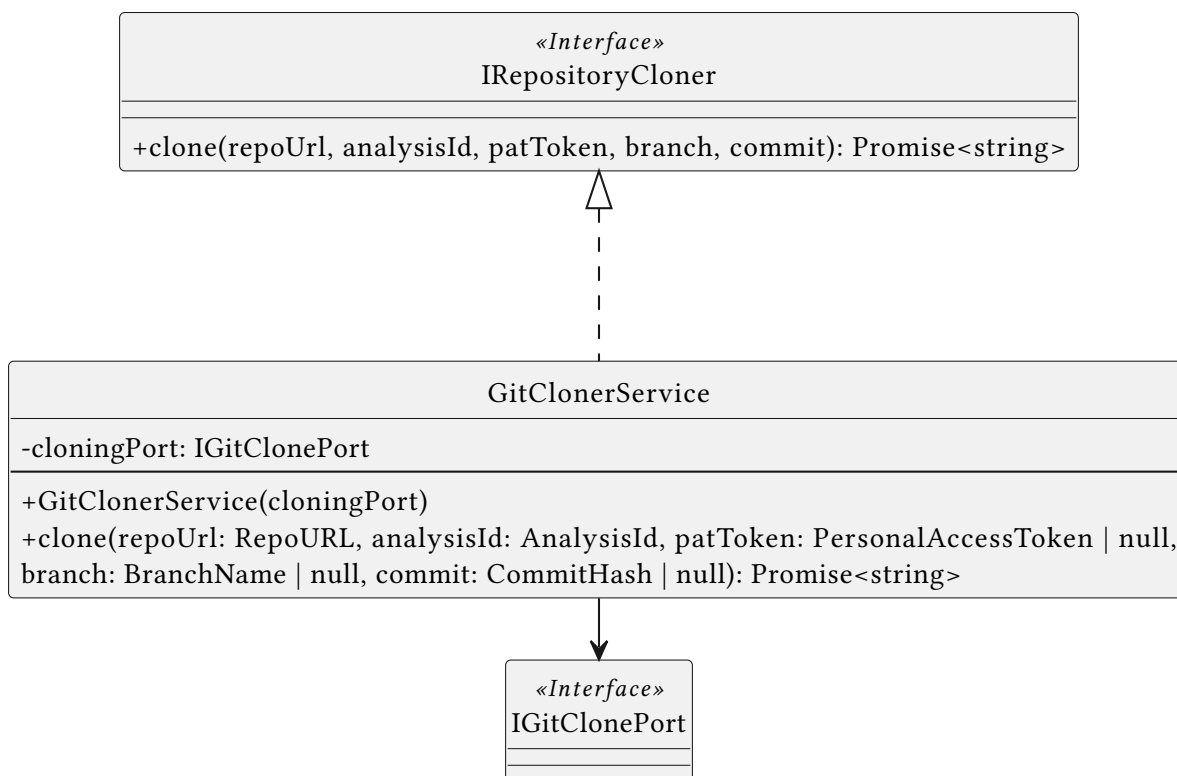
Figure 90: Class Diagram — GitClonerService
