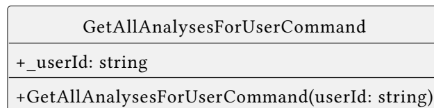
Figure 56: Class Diagram — GetAllAnalysesForUserCommand
