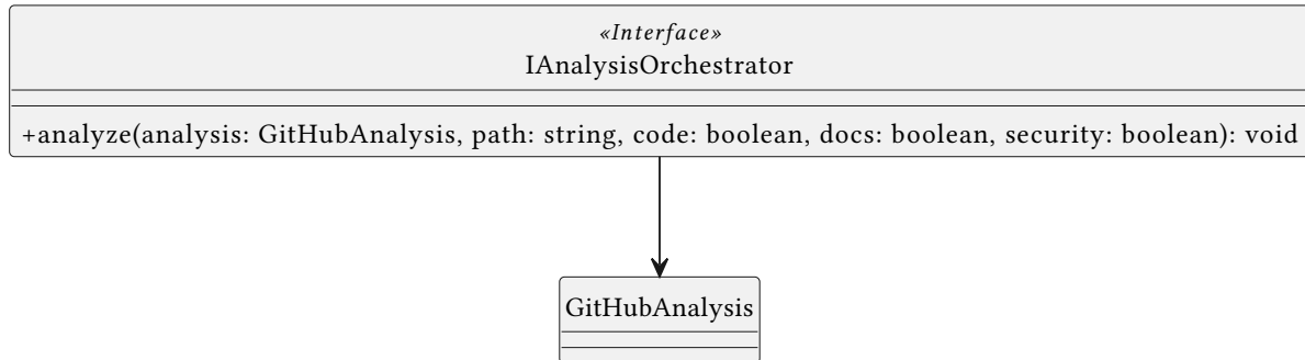
Figure 83: Class Diagram – IAnalysisOrchestrator
