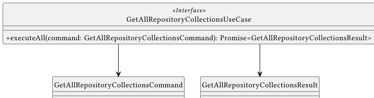
Figure 67: Class Diagram — GetAllRepositoryCollectionsUseCase
