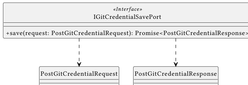
Figure 116: Class Diagram – IGitCredentialSavePort
