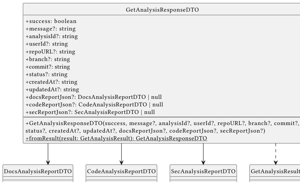
Figure 186: Class Diagram — GetAnalysisResponseDTO
