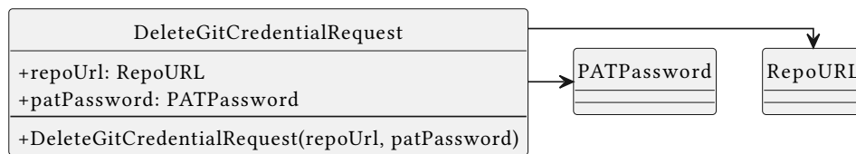
Figure 126: Class Diagram — DeleteGitCredentialRequest
