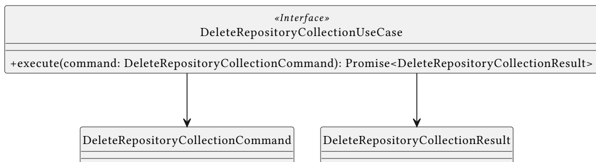
Figure 65: Class Diagram — DeleteRepositoryCollectionUseCase
