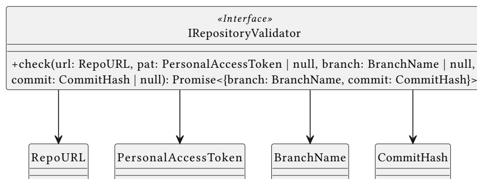
Figure 87: Class Diagram – IRepositoryValidator
