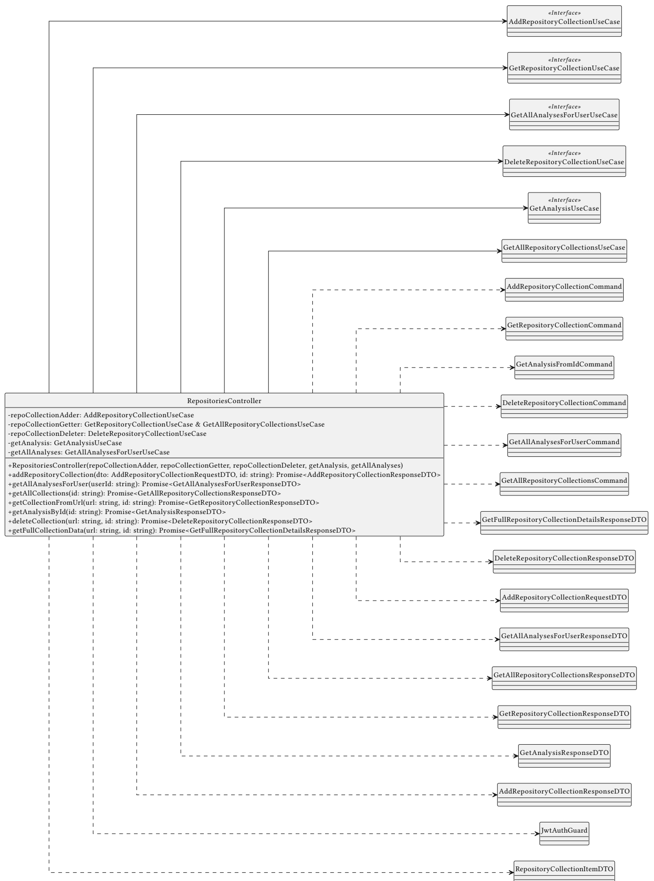
Figure 175: Class Diagram — RepositoriesController
