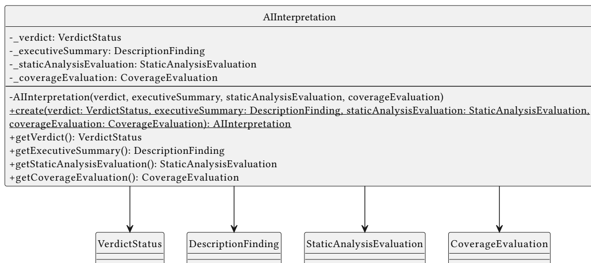
Figure 6: Class Diagram — AIInterpretation
