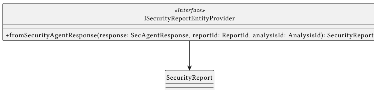
Figure 51: Class Diagram — ISecurityReportEntityProvider
