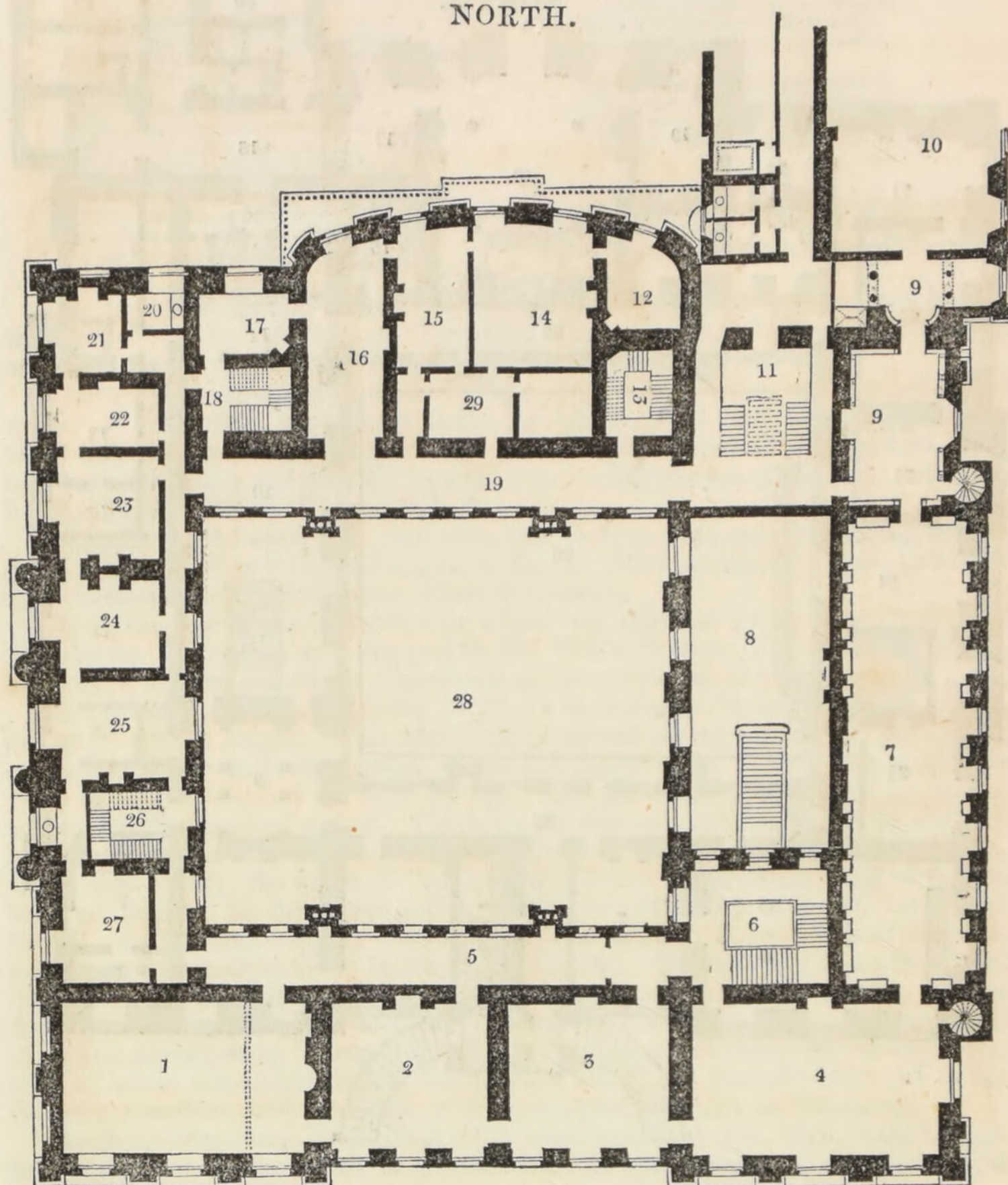
No. 2. Plan of the Library Story.
