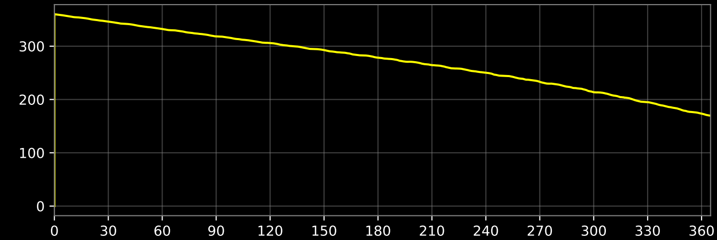
RAAN ( \Omega , grader)
