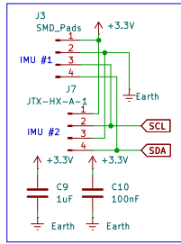
Main IMU
