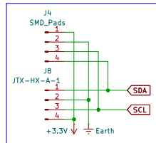
Extension IMU
