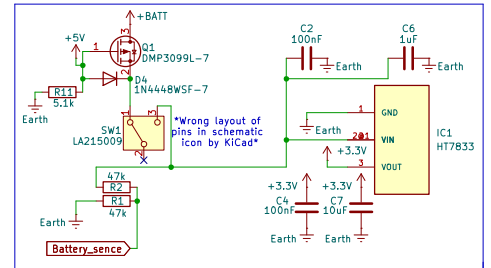
From +Batt to 3.3V
