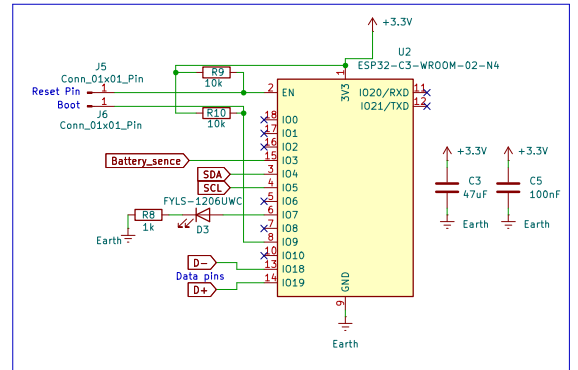
Main MCU
