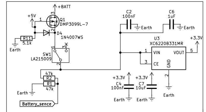
From +Batt to 3.3V
