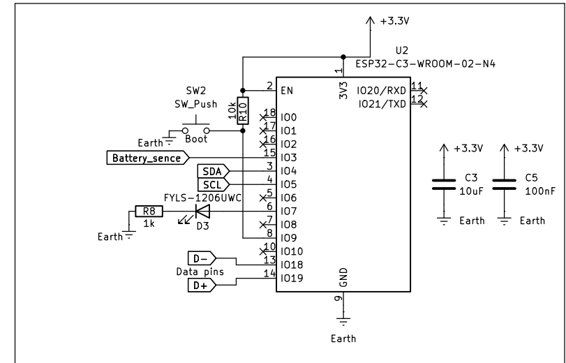
Main MCU
