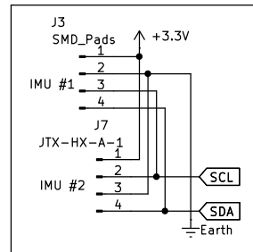
Main IMU
