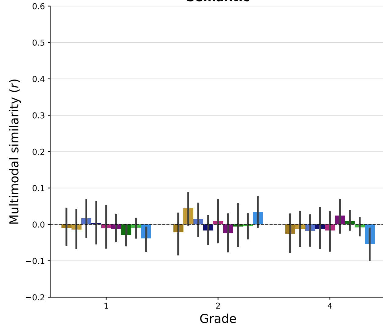
Semantic
