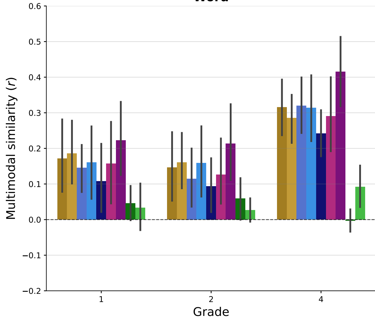
Word
