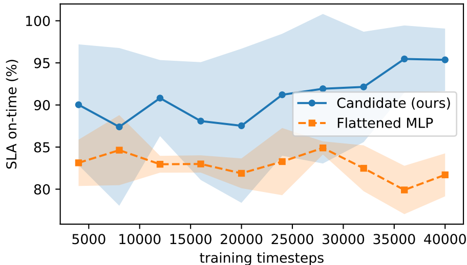
Learning curves (routed reward, standard\_tight)
