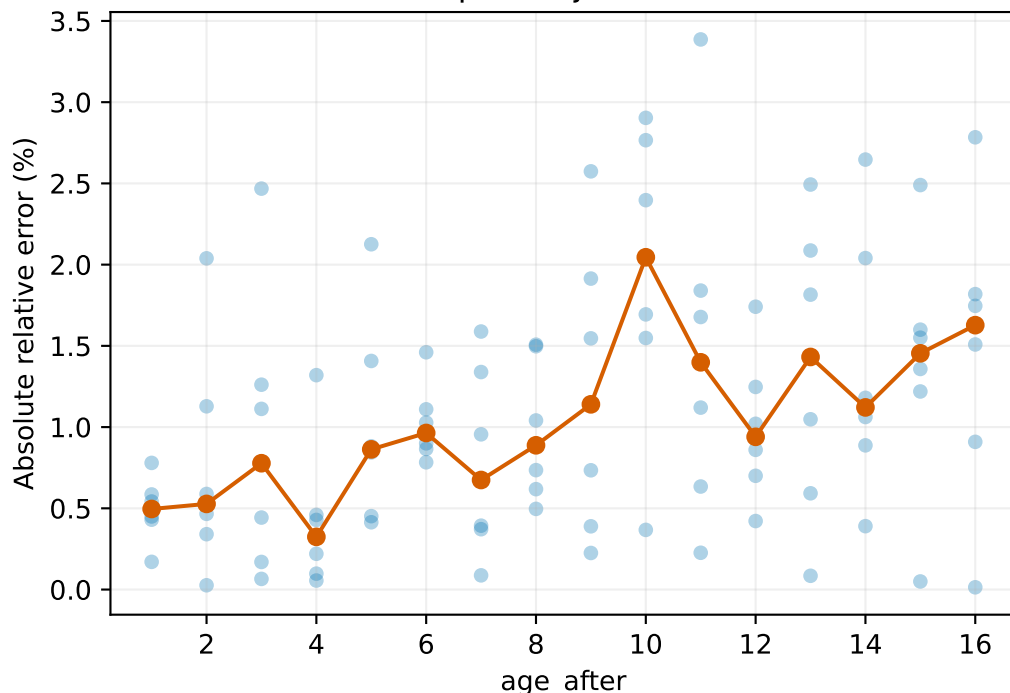
Cross-term approximation
