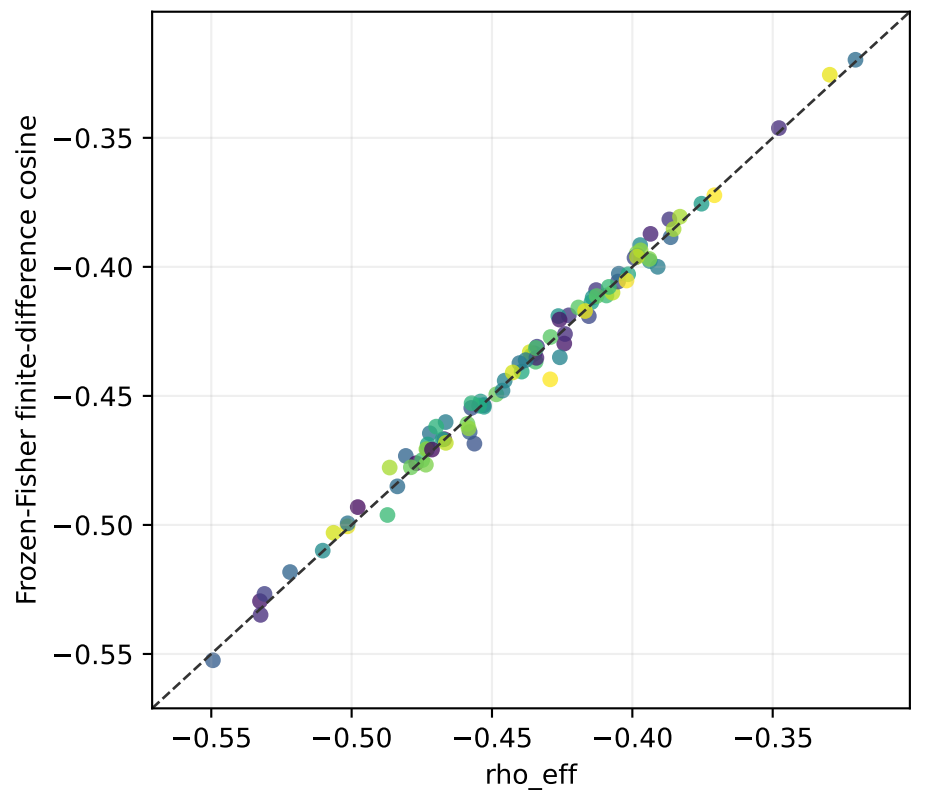
Finite-difference cosine vs effective rho
