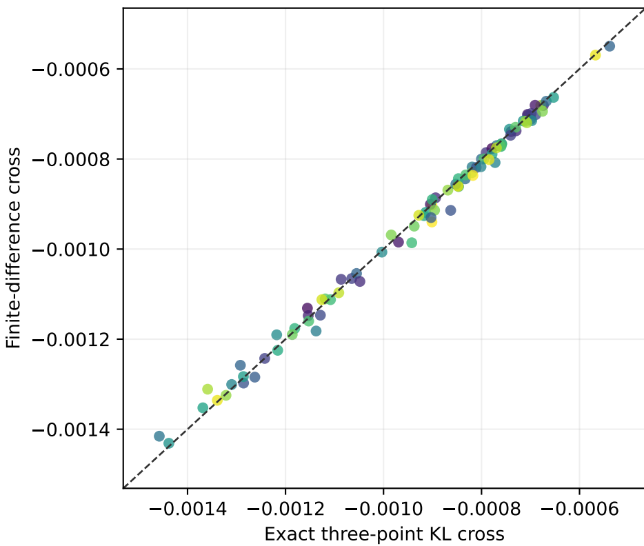
Finite-difference cross vs exact KL cross
