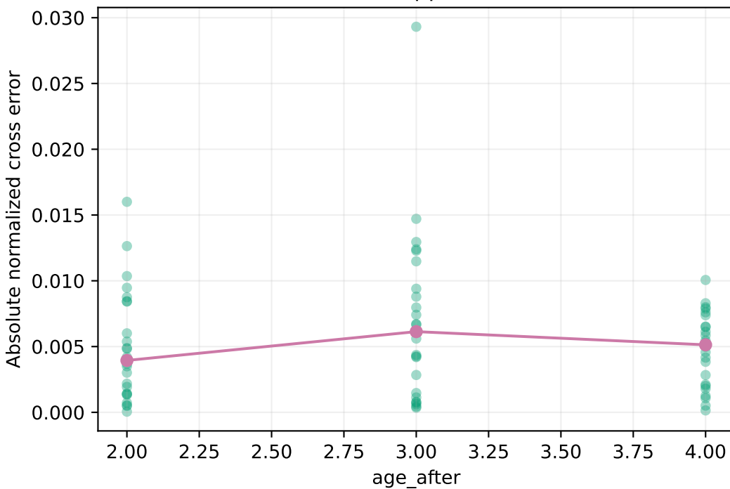
Cross-term approximation
