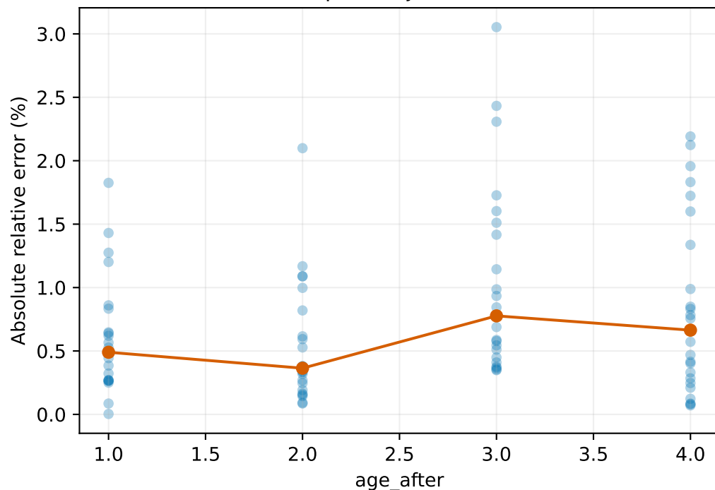
Cross-term approximation
