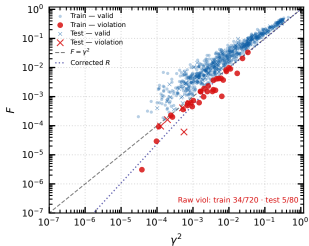
Brickwork L=5
