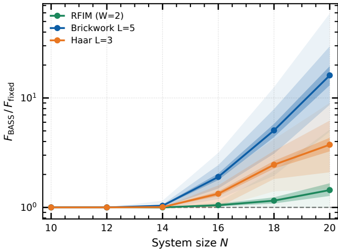
Fixed k = 8, 192
