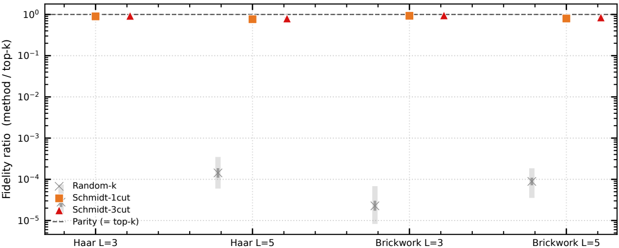
Schmidt truncation vs top-k: N=16, k=8192, 100 trials Dot = geomean · Medium bar = 95% bootstrap CI · Light bar = IQR
