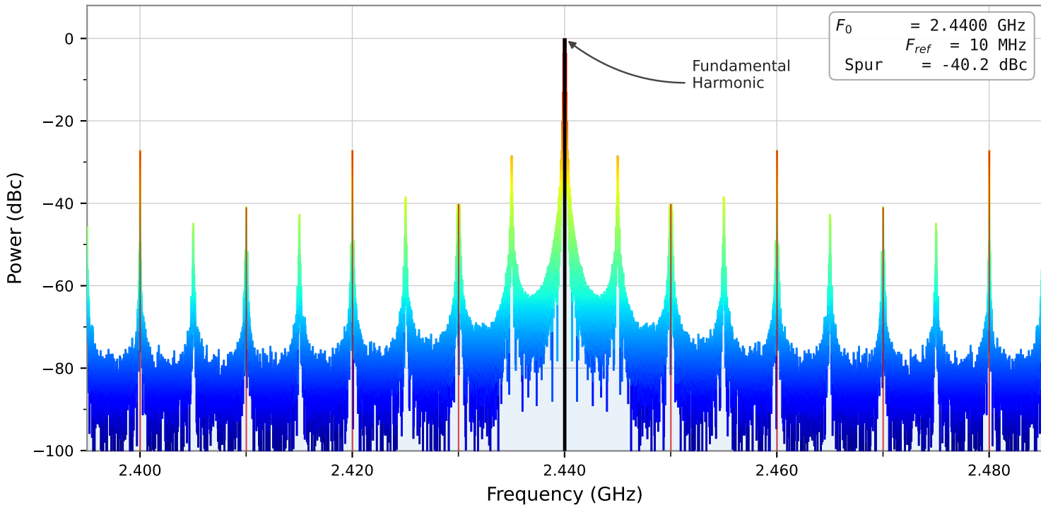
PLL Output Spectrum — Reference Spur: -40.2 dBc @ 10 MHz offset | f_0 = 2.4400 GHz
