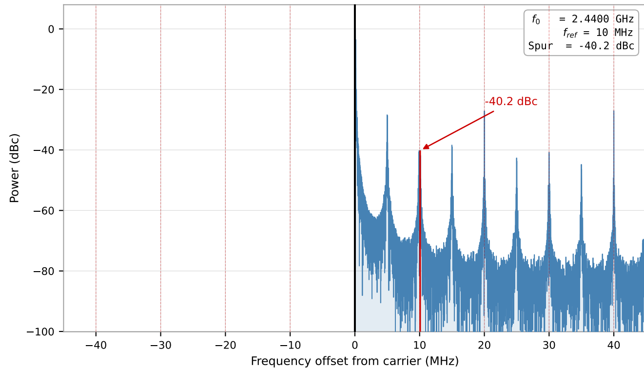
Method A — Zero-crossing jitter FFT (same as plot_reference_spur.py)
