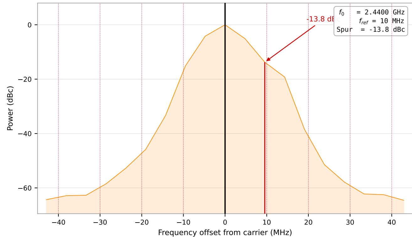
Method B — Welch PSD on raw v(clk_out) (independent verification)
