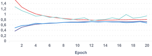
training_history / LinePlot
