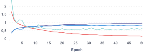
training_history_improved / LinePlot
