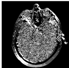
Quantized Directions
