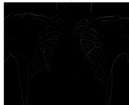
Non-Max Suppression
