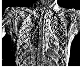
Non-Max Suppression
