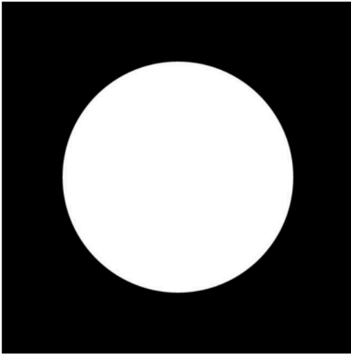
NMS Result
