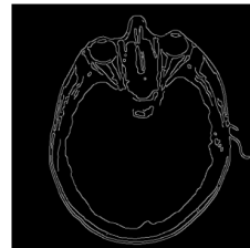
Final Edges
