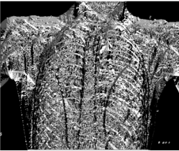
Quantized Directions
