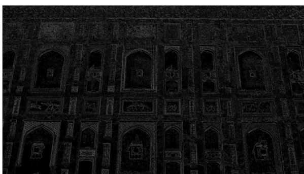
NMS Result
