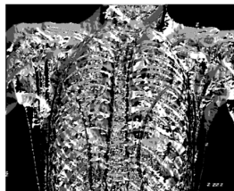
Quantized Directions
