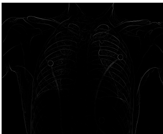
NMS Result
