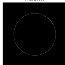
Final Edges
