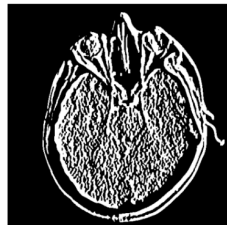
Non-Max Suppression
