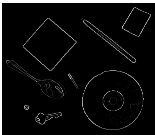
NMS Result
