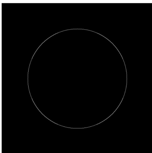
NMS Result
