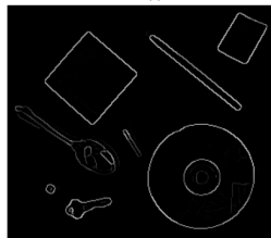
Non-Max Suppression
