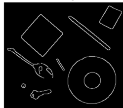
Final Edges
