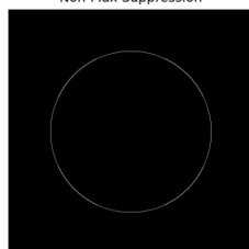
Non-Max Suppression
