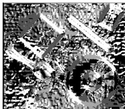
Quantized Directions
