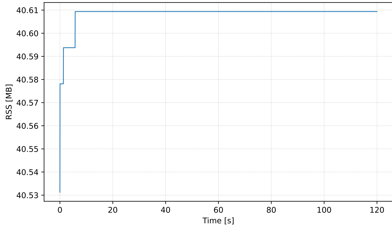
RPi5 Edge Benchmark — 50.0Hz — RSS vs Time
