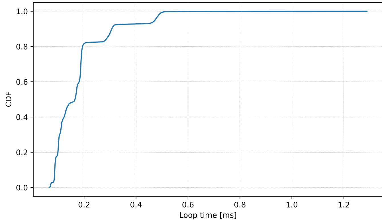
Control Loop Time CDF
