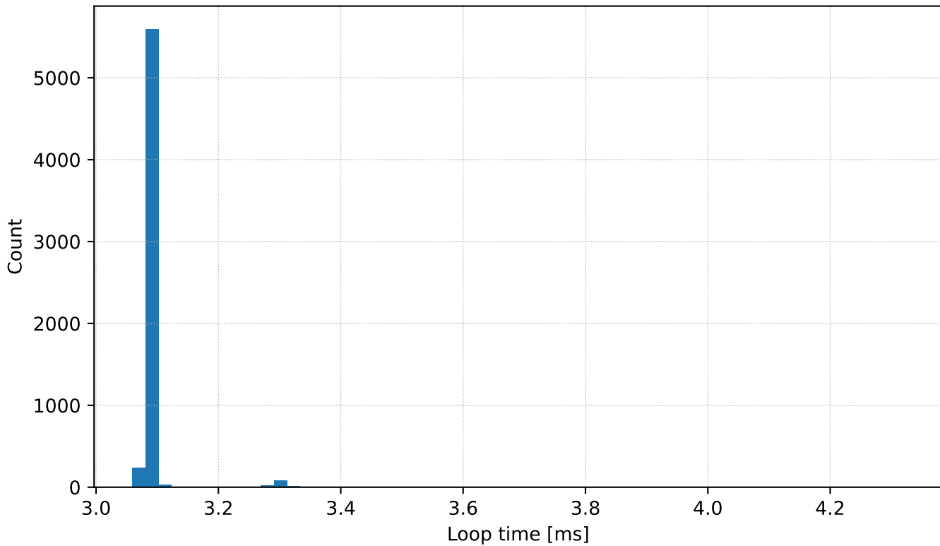
RPi5 Edge Benchmark — 50.0Hz — Loop Histogram
