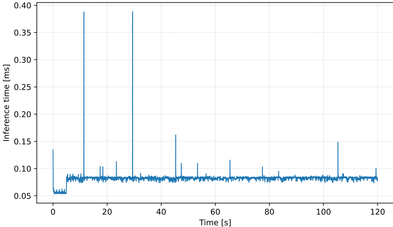
RPi5 Edge Benchmark — 50.0Hz — Inference vs Time
