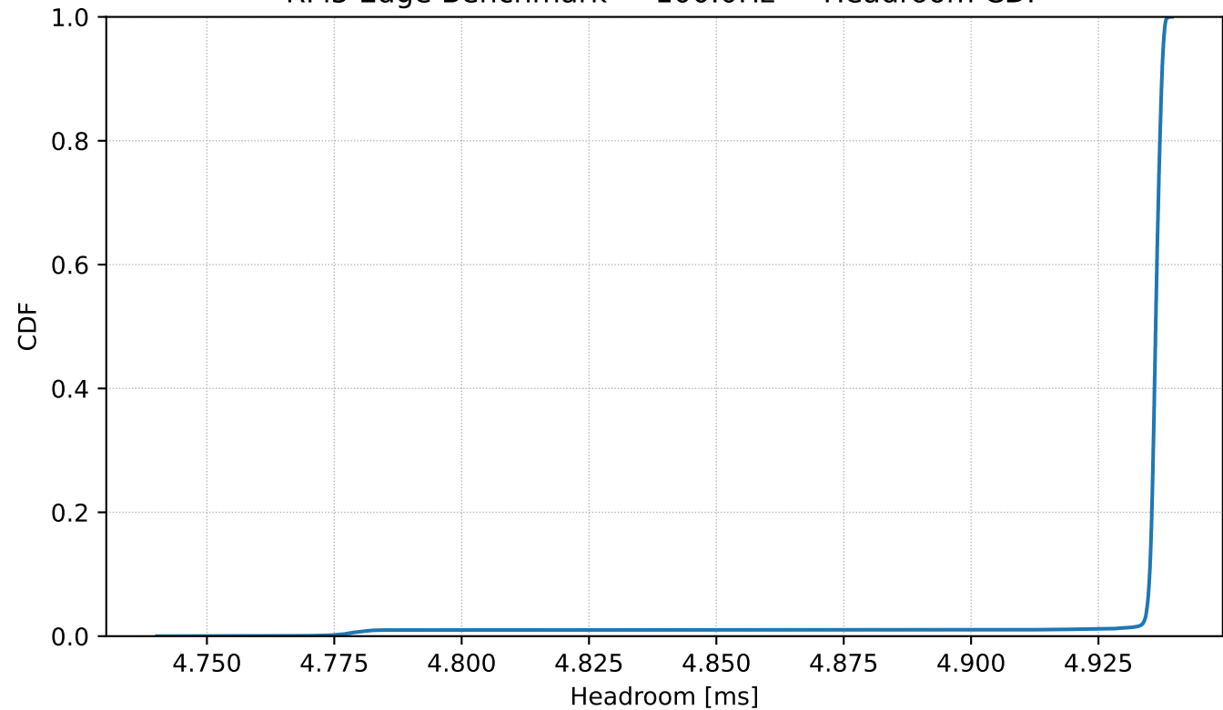
RPi5 Edge Benchmark — 100.0Hz — Headroom CDF
