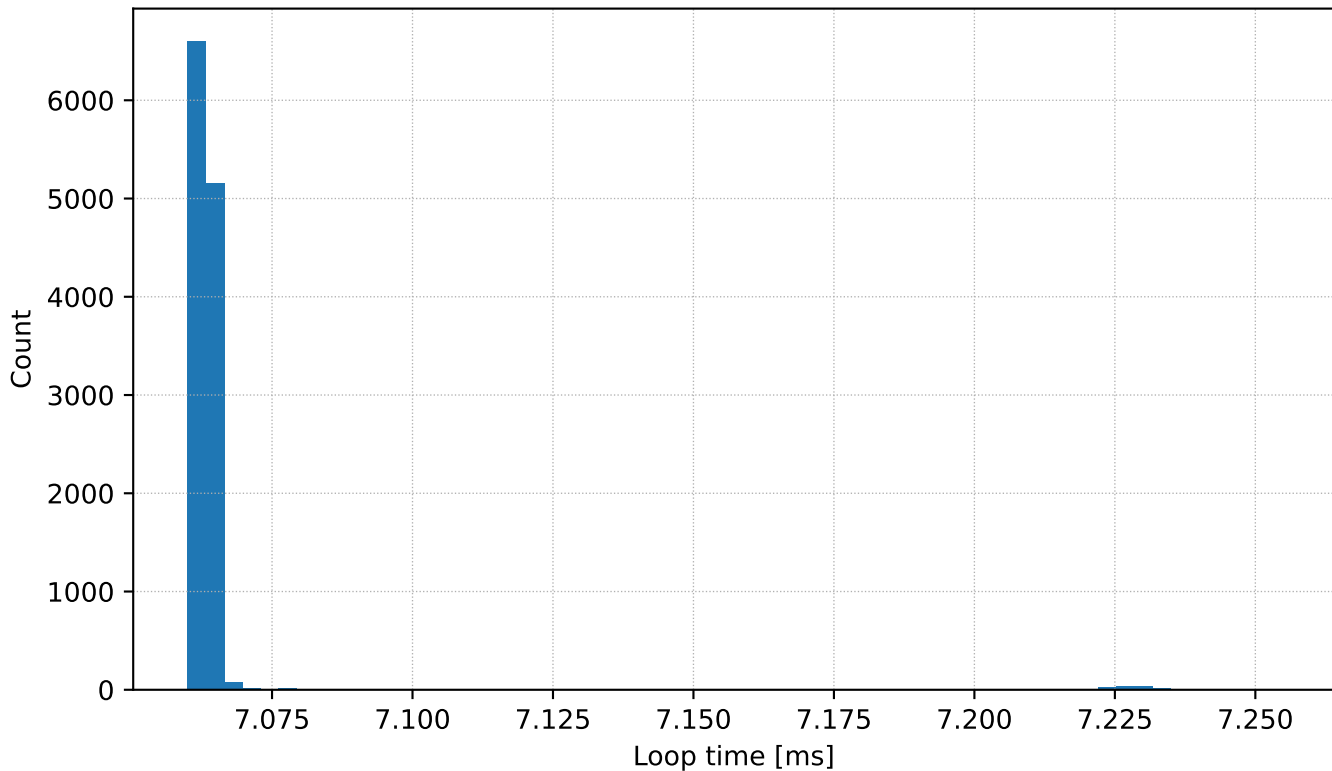
RPi5 Edge Benchmark — 100.0Hz — Loop Histogram
