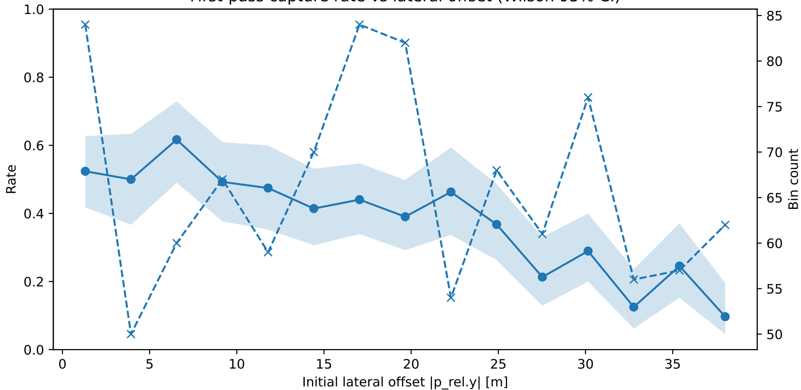
First-pass capture rate vs lateral offset (Wilson 95% CI)
