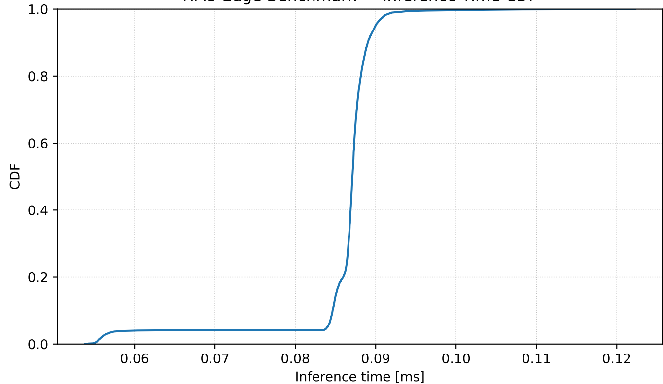
RPi5 Edge Benchmark — Inference Time CDF
