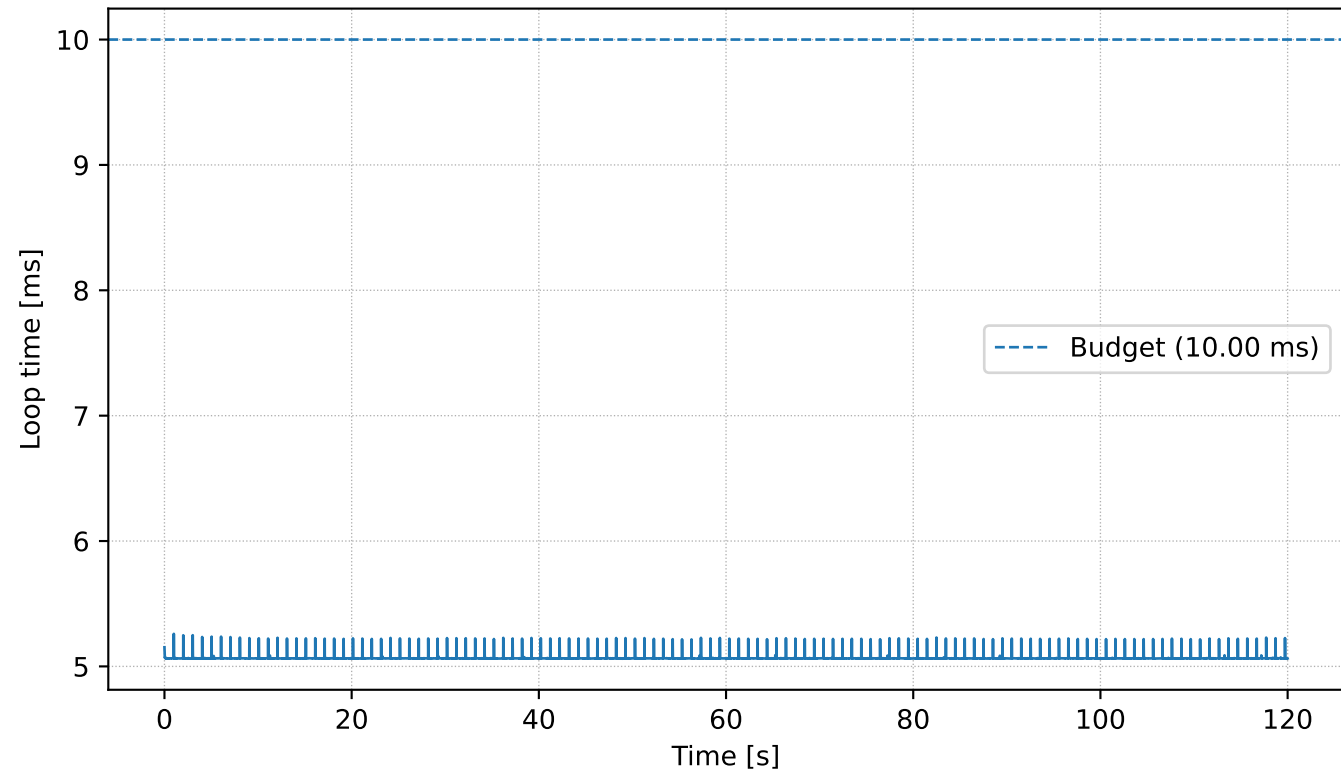
RPi5 Edge Benchmark — 100.0Hz — Loop vs Time
