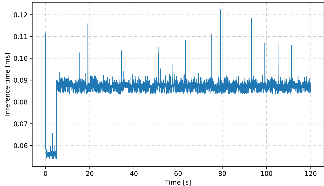
RPi5 Edge Benchmark — Inference Time vs Time
