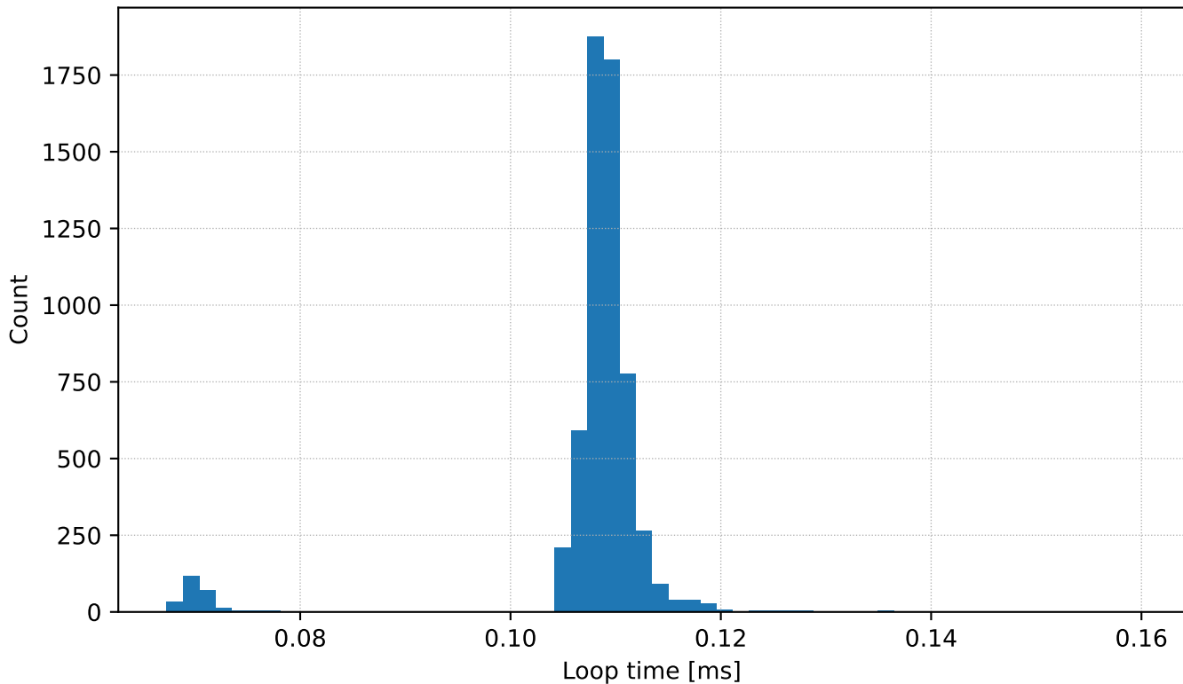
RPi5 Edge Benchmark — Loop Time Histogram
