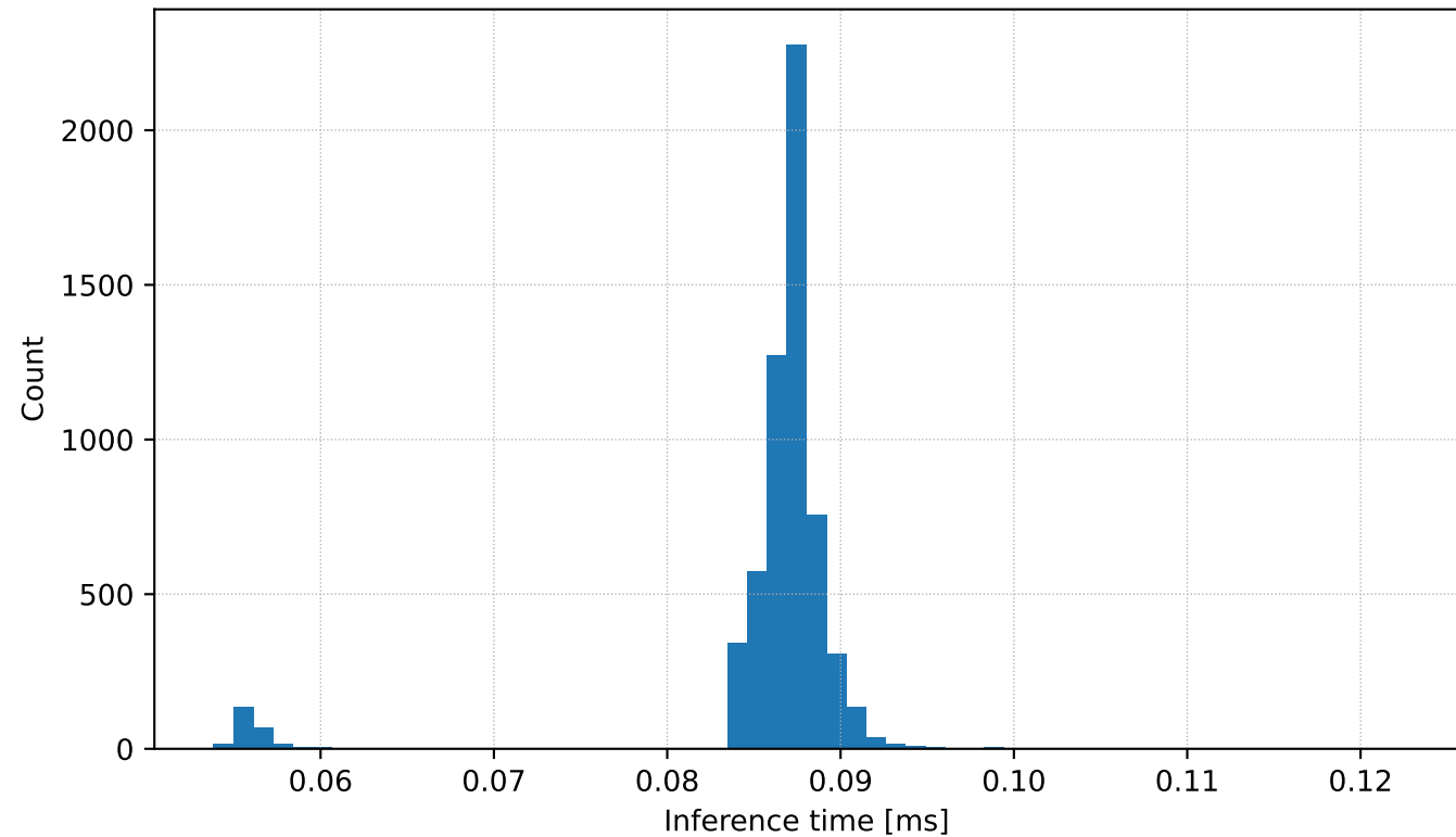
RPi5 Edge Benchmark — Inference Time Histogram
