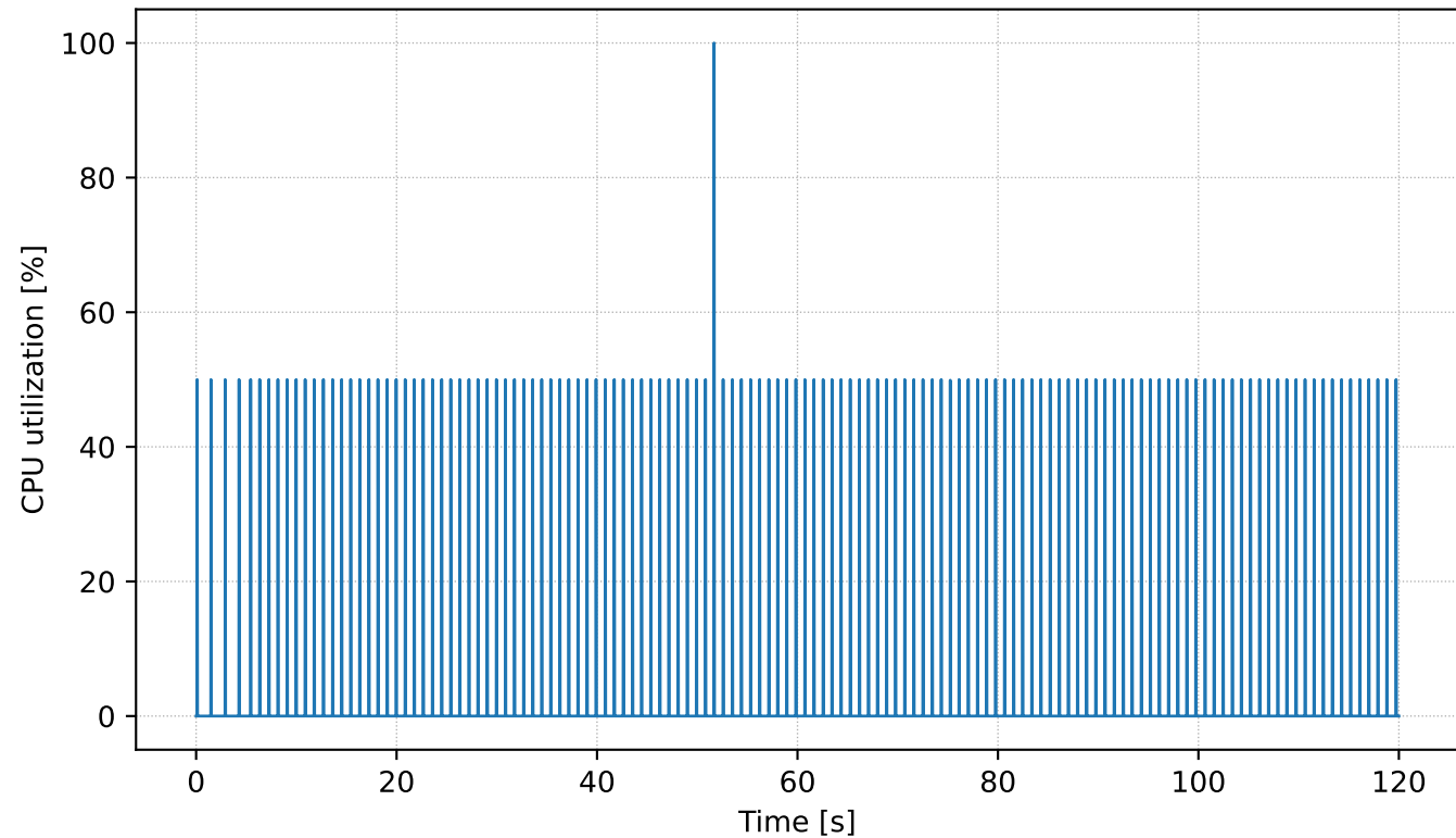
RPi5 Edge Benchmark — CPU Utilization vs Time
