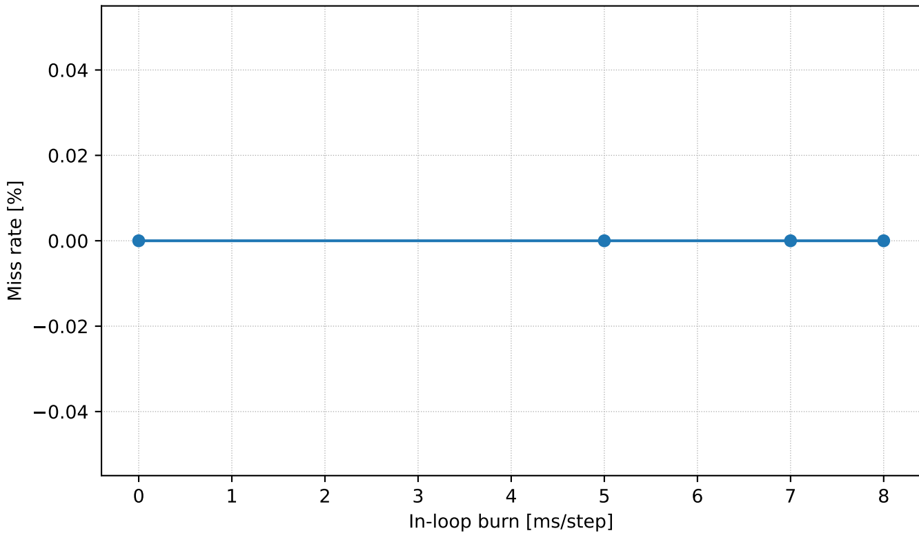
Deadline Miss Rate vs Added In-loop Workload (100 Hz)
