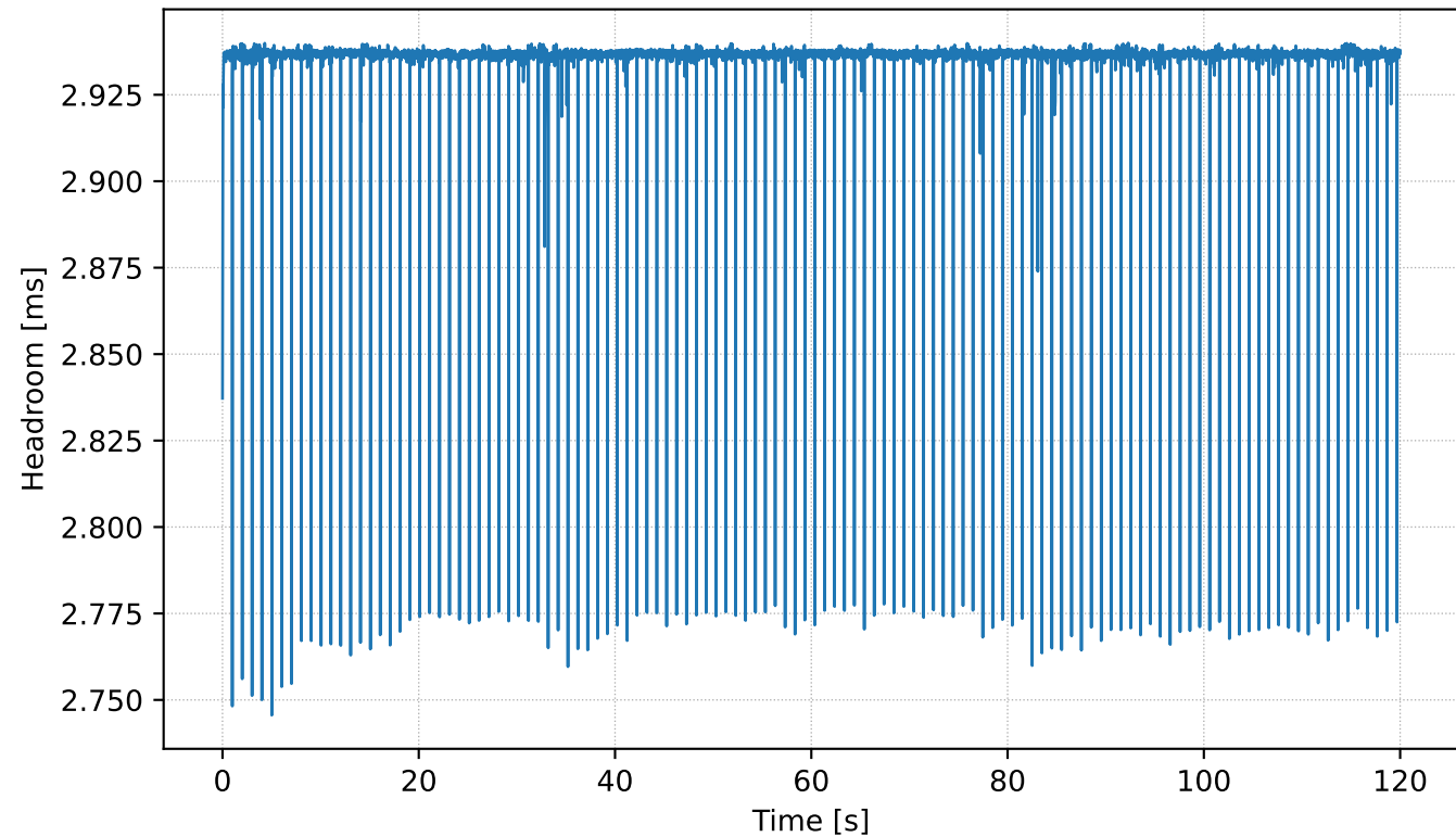
RPi5 Edge Benchmark — 100.0Hz — Headroom vs Time
