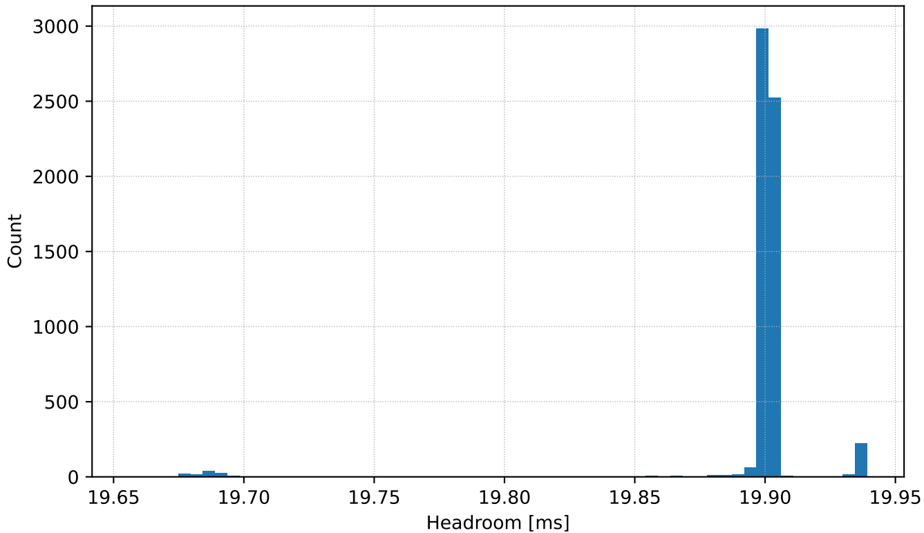
RPi5 Edge Benchmark — 50.0Hz — Headroom Histogram
