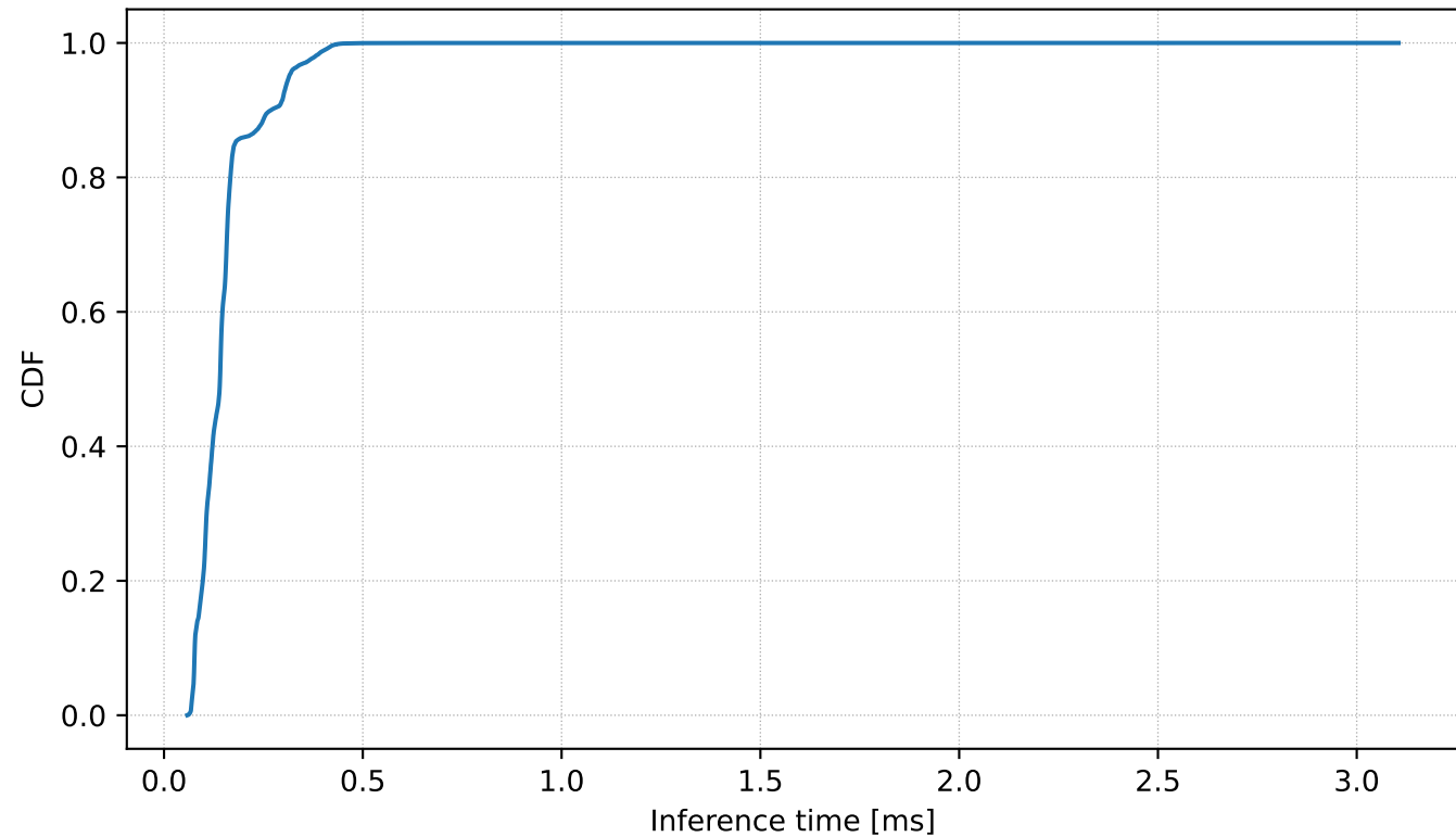
Inference Time CDF
