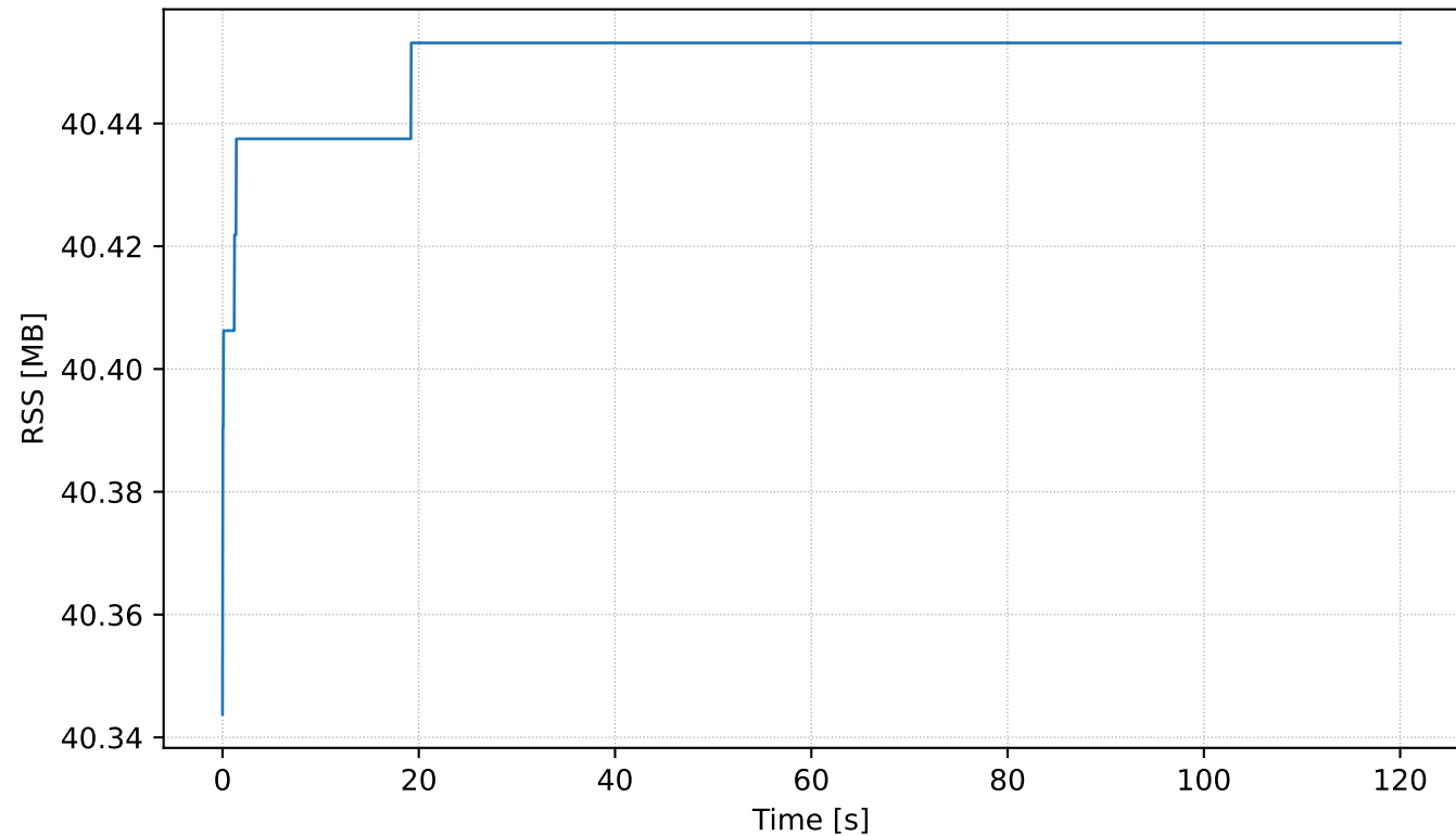
RPi5 Edge Benchmark — 100.0Hz — RSS vs Time
