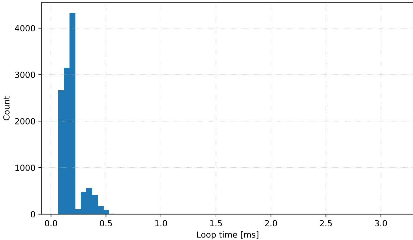
Control Loop Time Histogram
