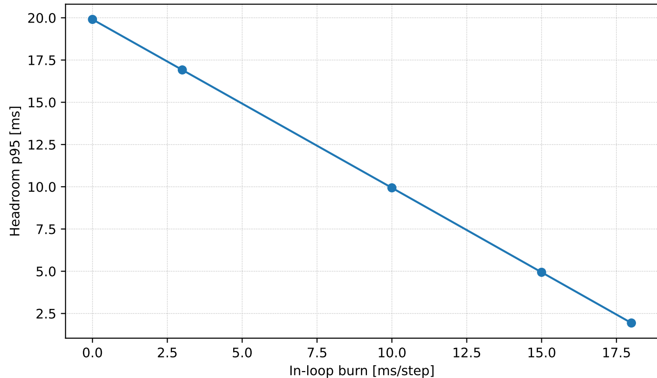
Headroom (p95) vs Added In-loop Workload (50 Hz)
