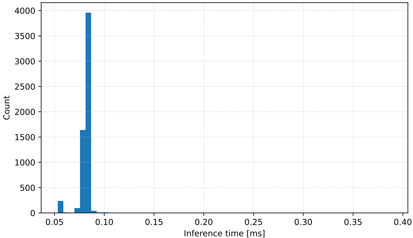
RPi5 Edge Benchmark — 50.0Hz — Inference Histogram
