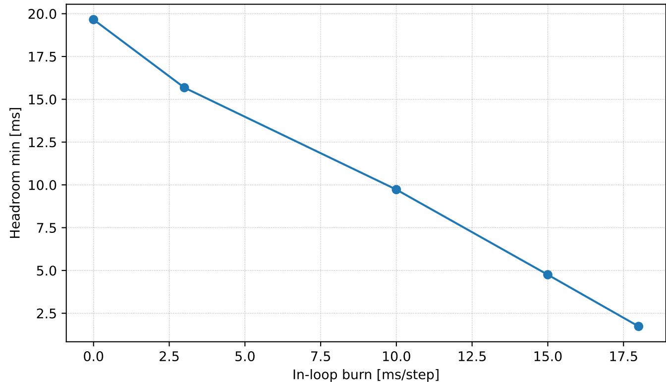
Headroom (min) vs Added In-loop Workload (50 Hz)
