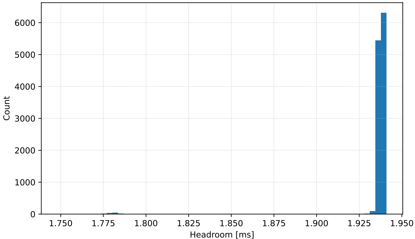
RPi5 Edge Benchmark — 100.0Hz — Headroom Histogram
