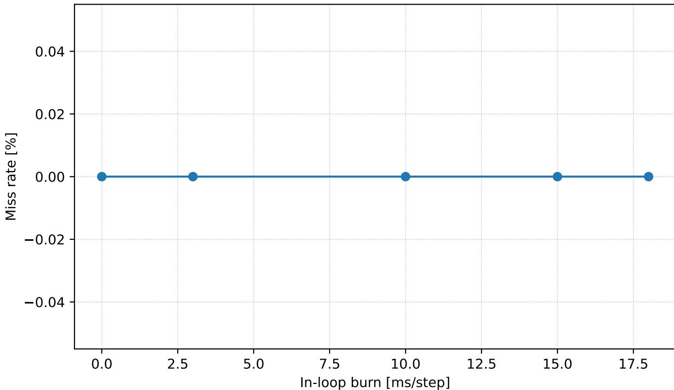
Deadline Miss Rate vs Added In-loop Workload (50 Hz)
