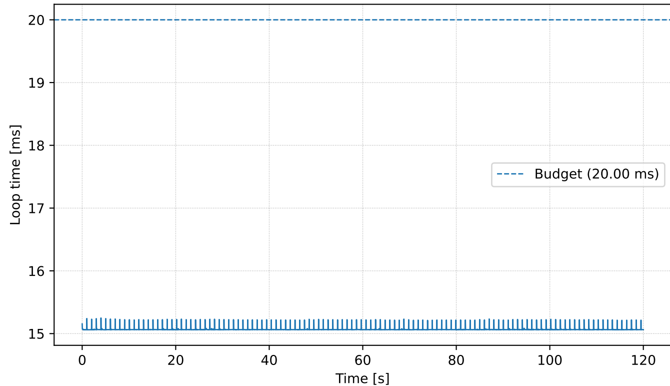
RPi5 Edge Benchmark — 50.0Hz — Loop vs Time
