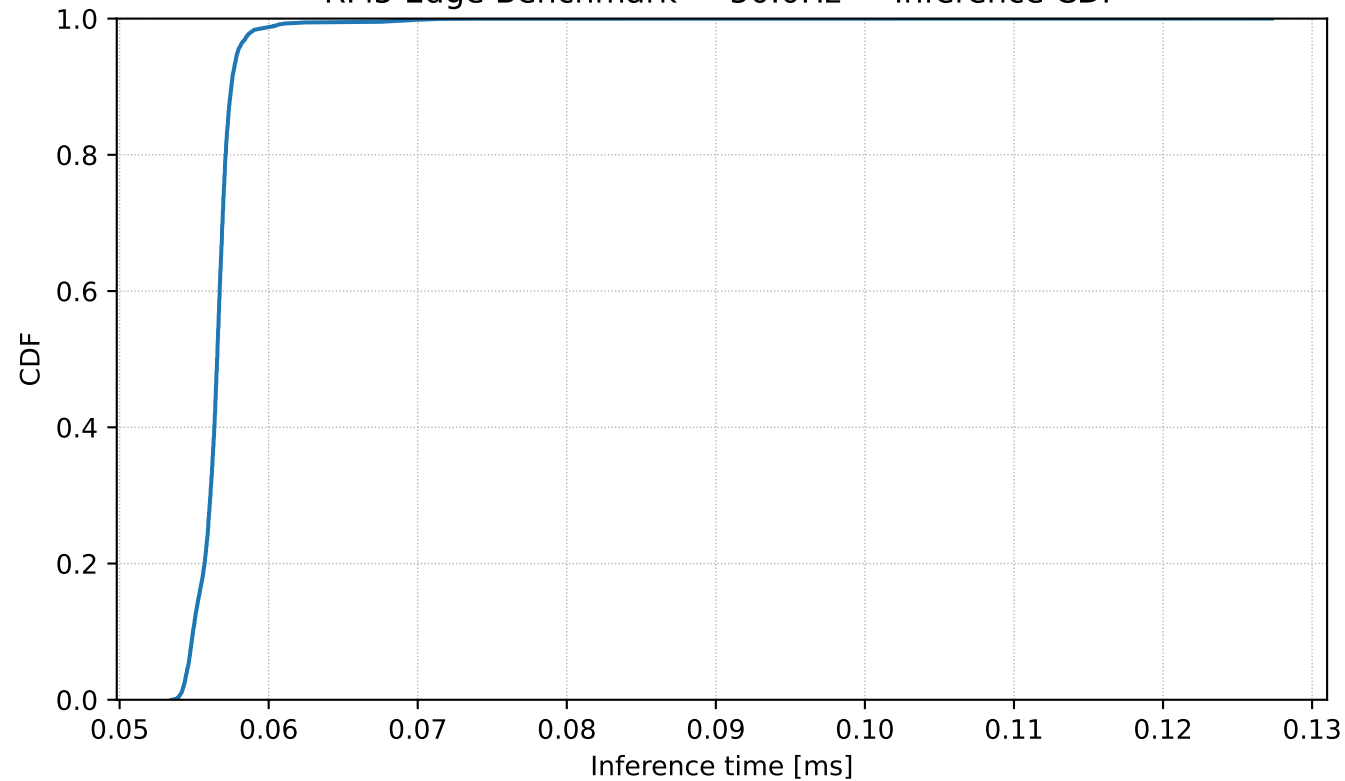
RPi5 Edge Benchmark — 50.0Hz — Inference CDF
