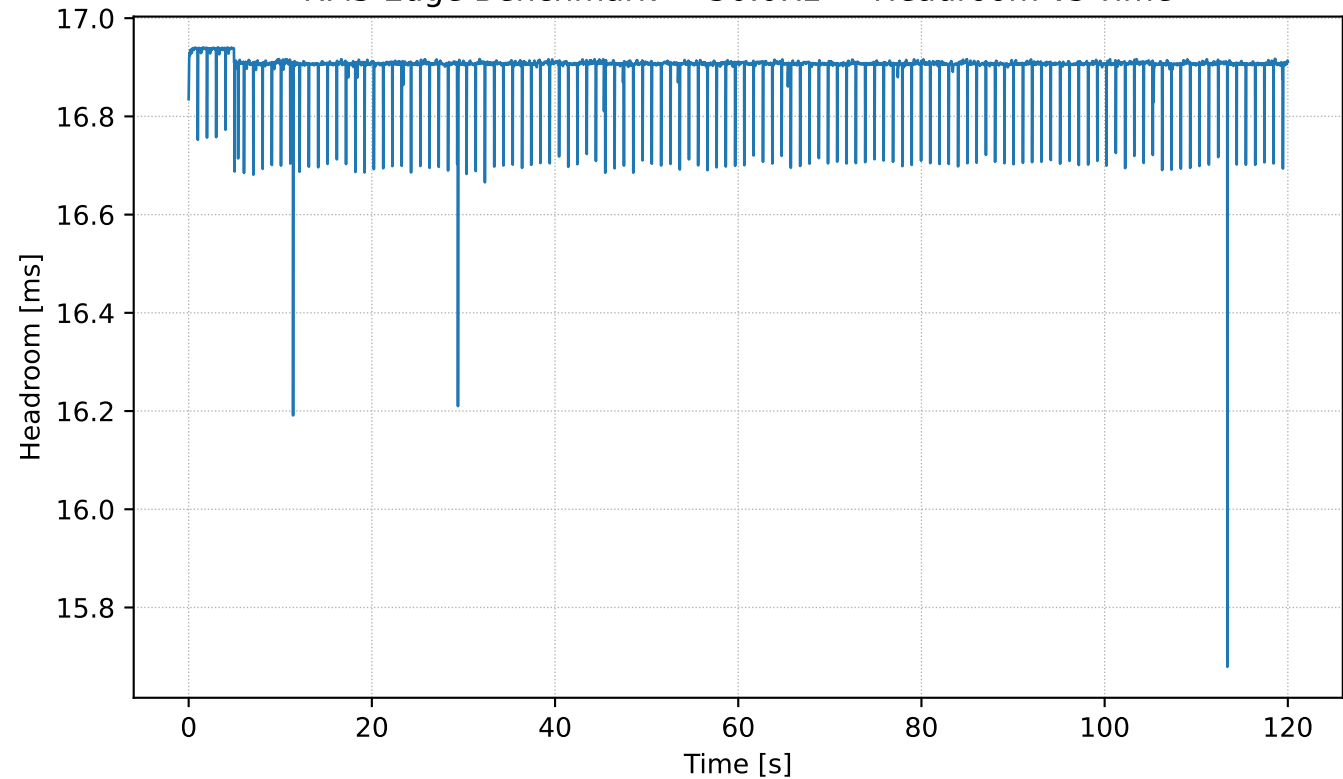
RPi5 Edge Benchmark — 50.0Hz — Headroom vs Time
