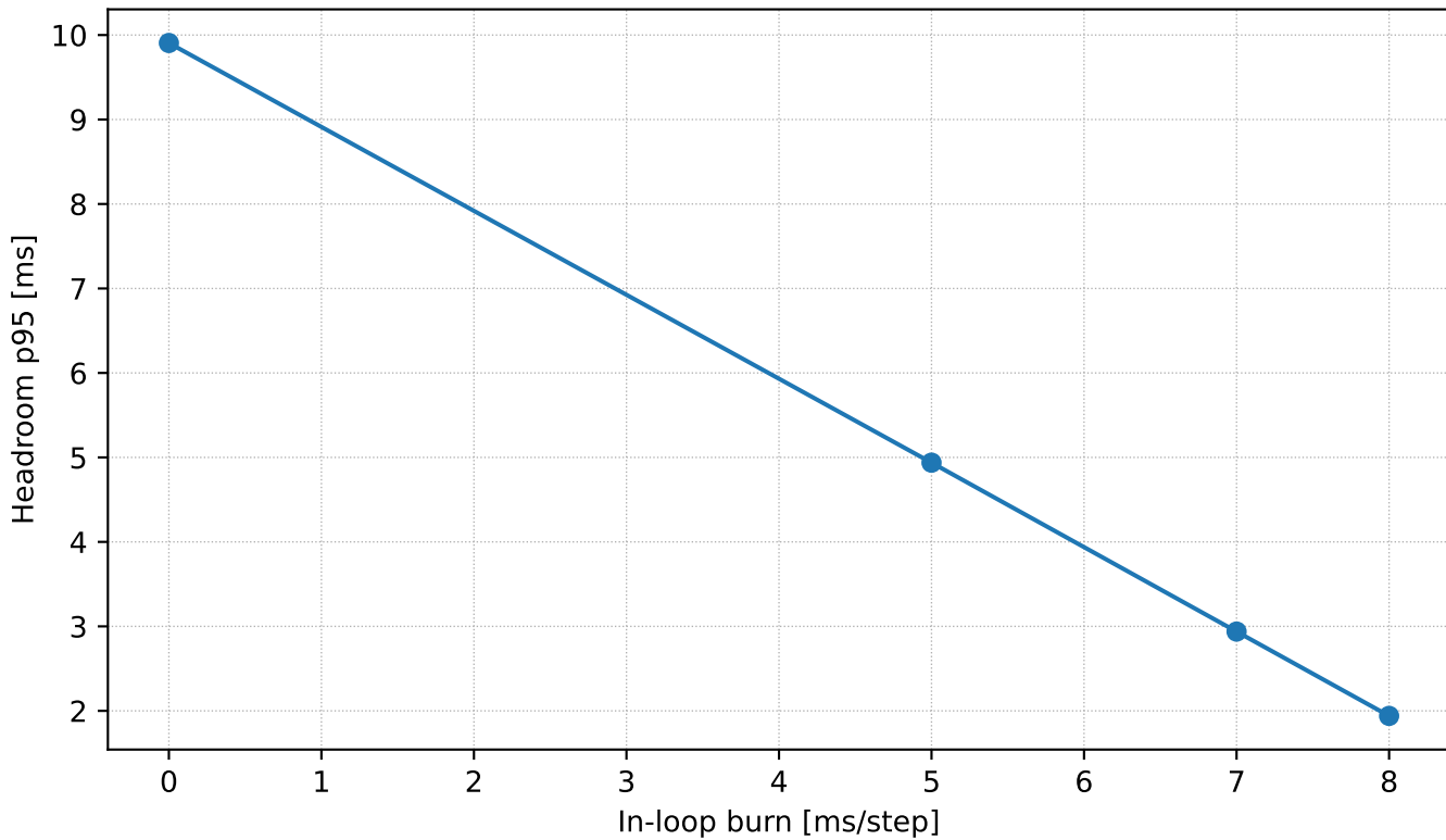
Headroom (p95) vs Added In-loop Workload (100 Hz)
