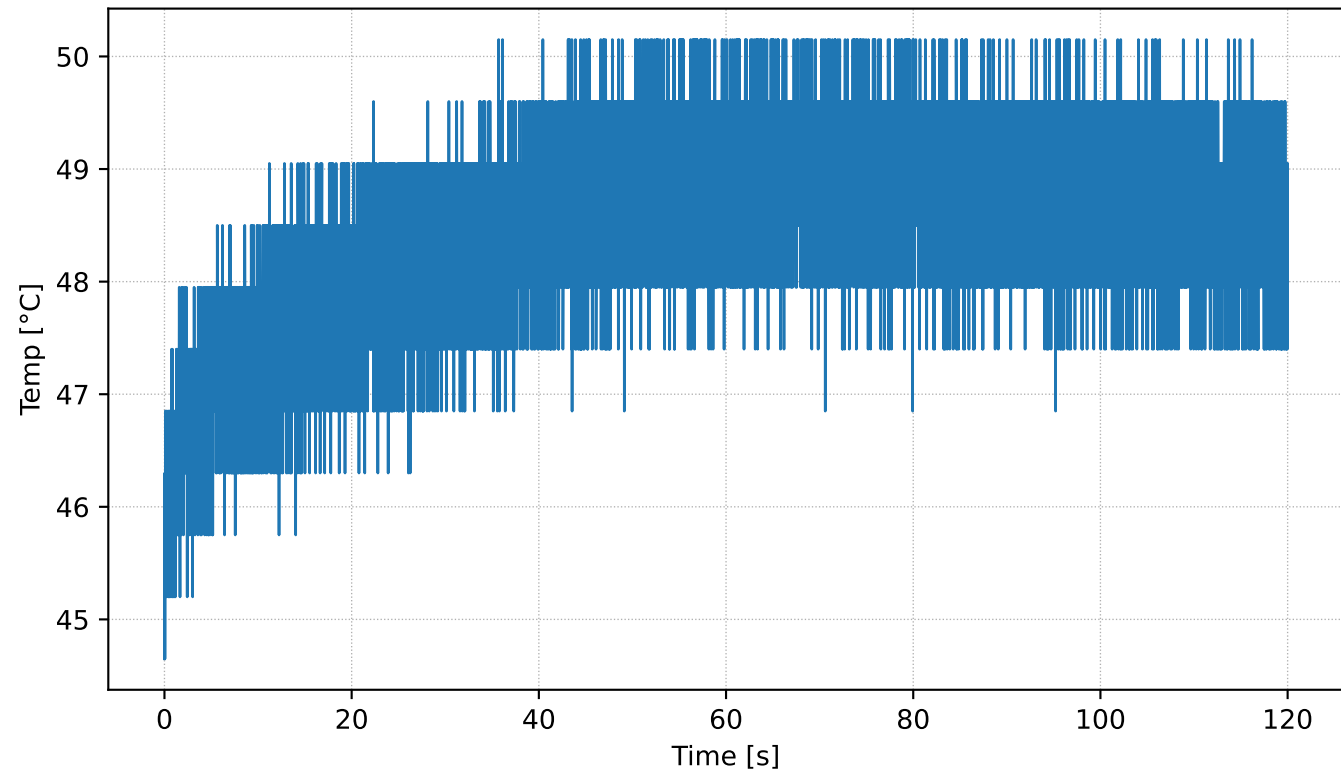
RPi5 Edge Benchmark — 100.0Hz — Temperature vs Time
