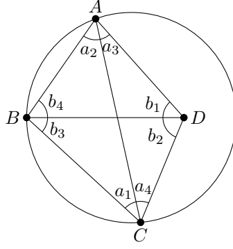
Figure 8: Angle labels used in Lemma 3
