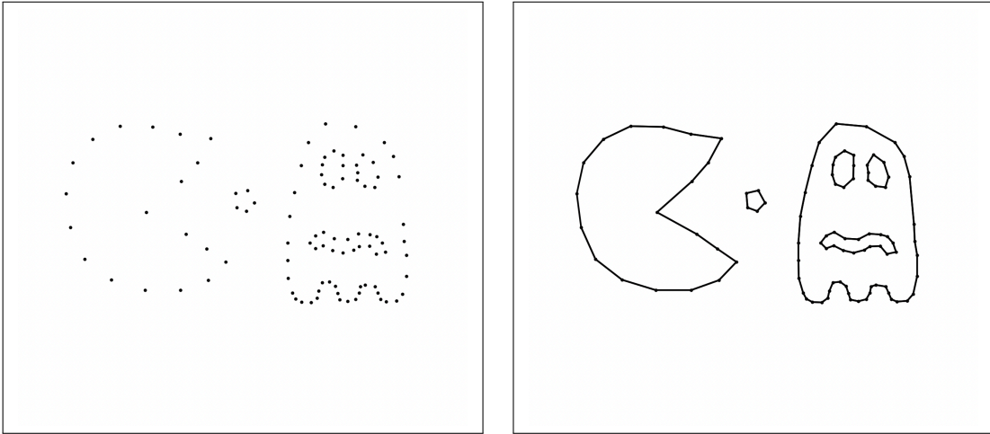
Figure 1: An example of the crust on a discrete set of points;
