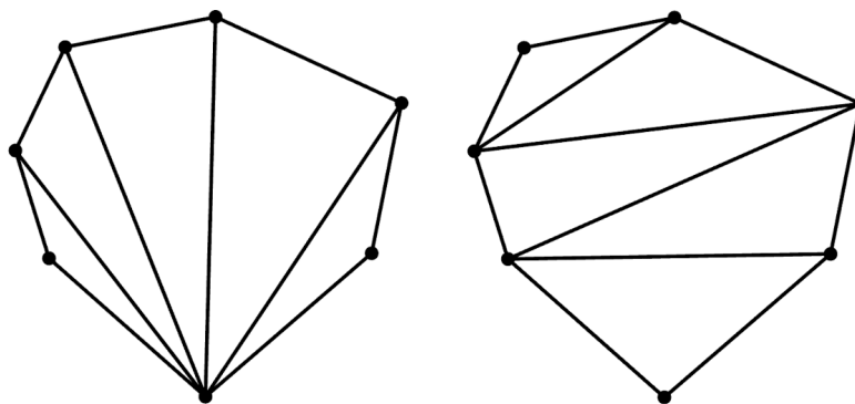
Figure 3: Two triangulations of a convex shape
