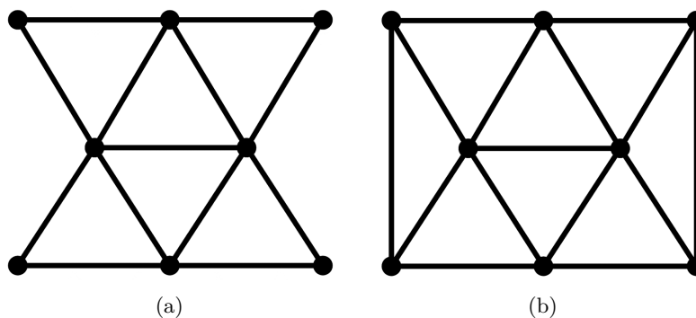
Figure 5: Two triangular meshes connecting the same set of points, showing the need for a maximal set.
