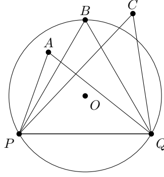
Figure 7: Three points with the same central angle inside, on, and outside the circle
