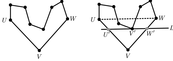
Figure 4: An example of how to show find a diagonal exists used in Lemma ??
