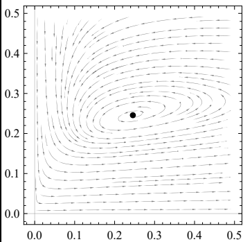
Foco inestable
