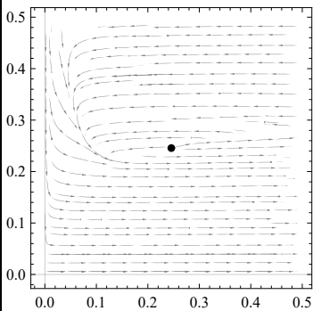
Nodo inestable
