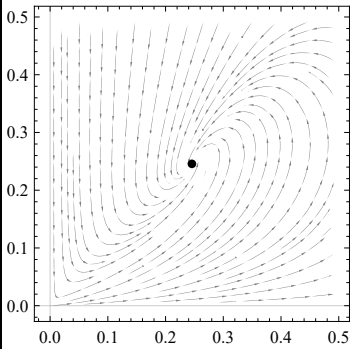
Foco estable
